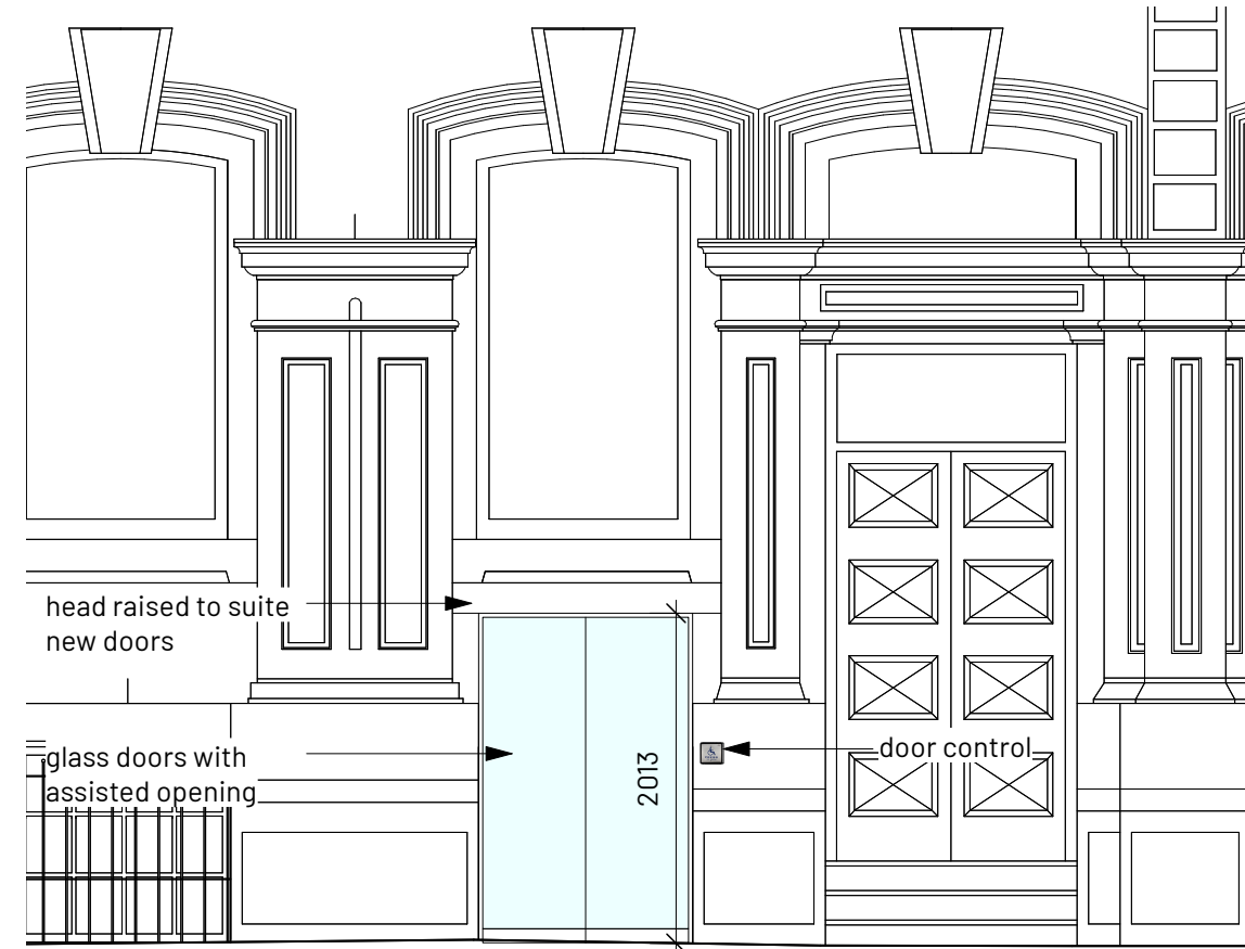
Unit A Princess Street Entrance - Elevation Scale: 1:50
