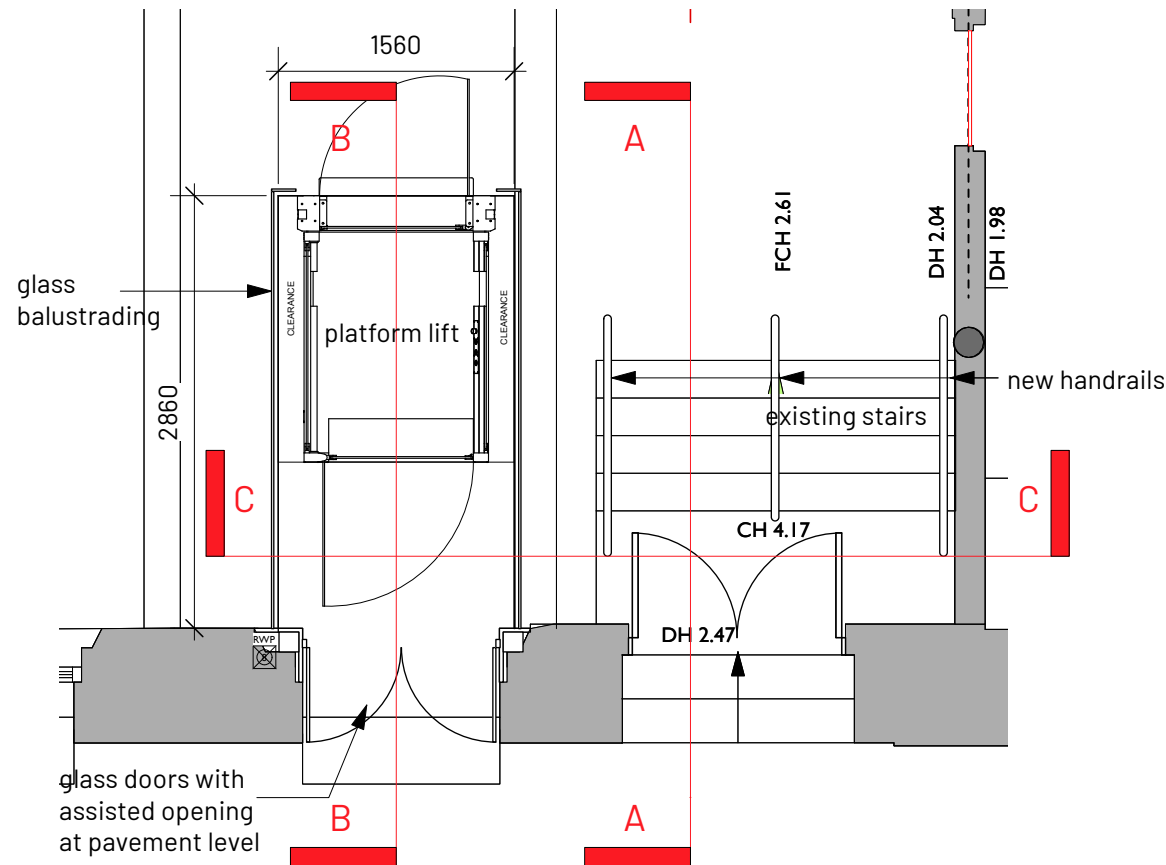
Unit A Princess Street Entrance - Plan Scale: 1:50
