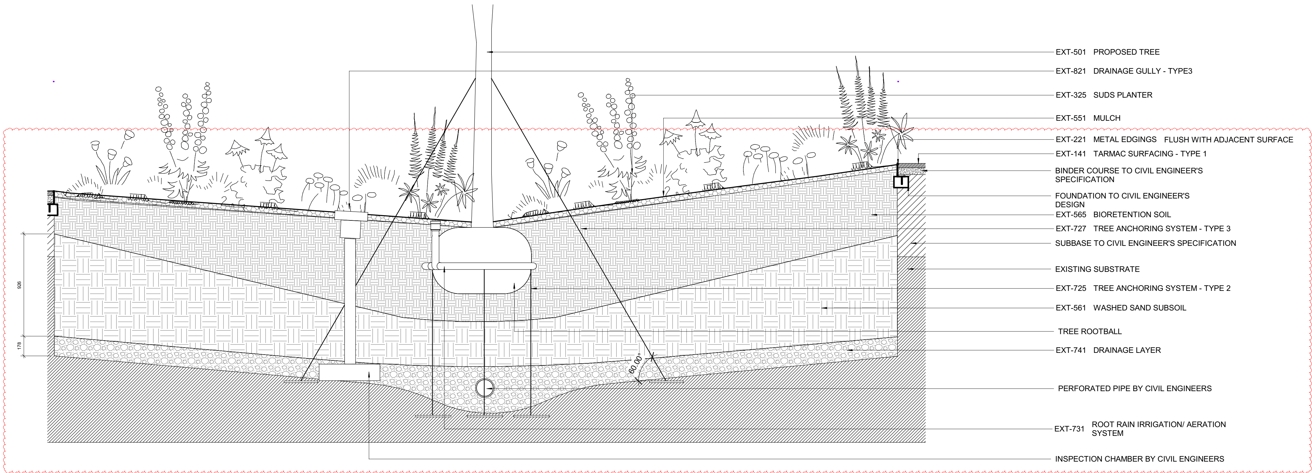
1 TYPICAL BIORETENTION PLANTER 1:20
