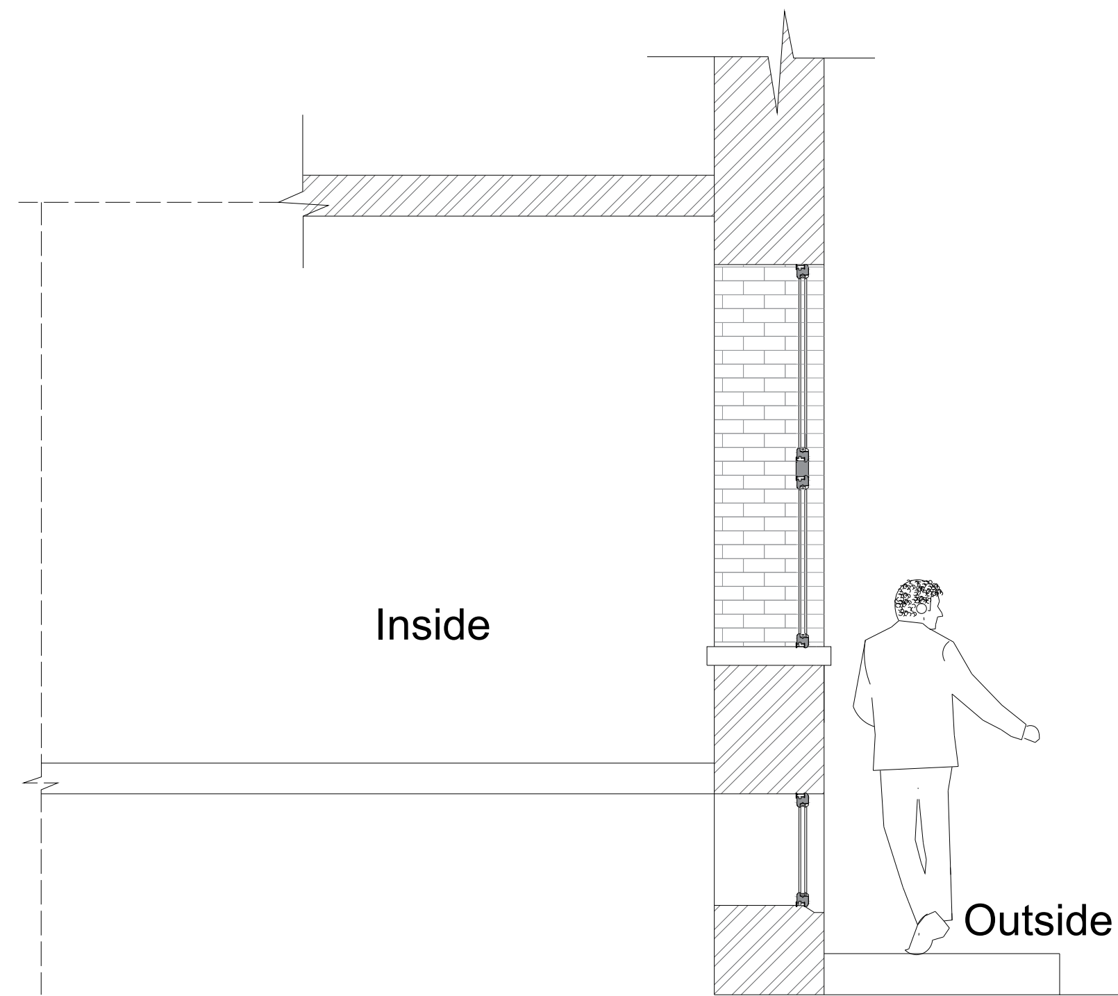
Existing section
