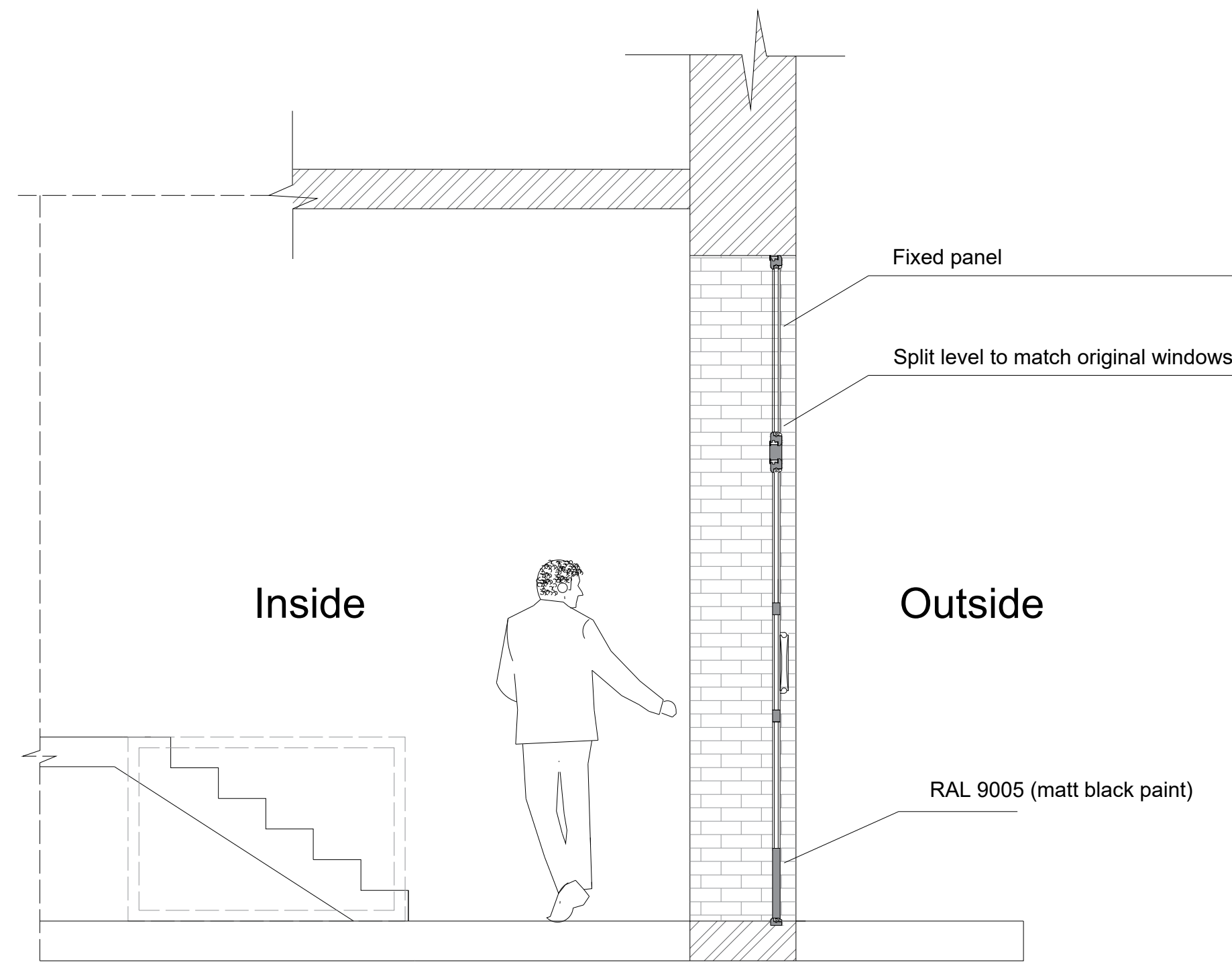
Proposed section AA for heritage Crittall style steel door
