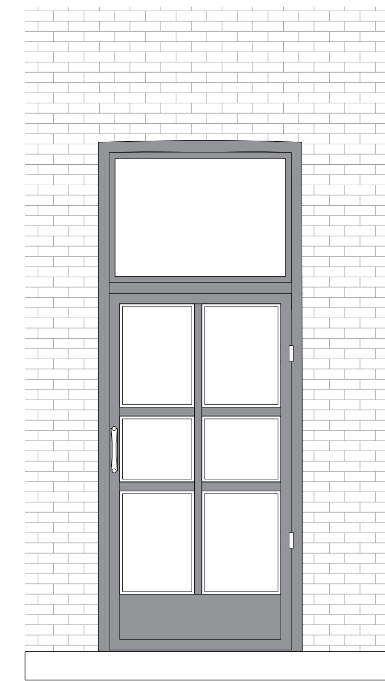
Proposed custom made crittall style steel door
