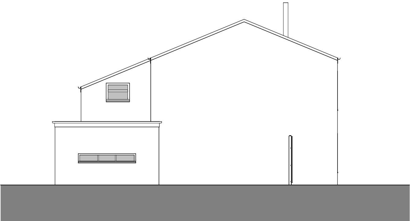
Planning - Existing Side Elevation B 1 : 100
