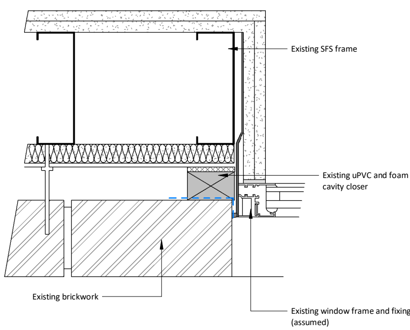
Window Jamb as Existing
