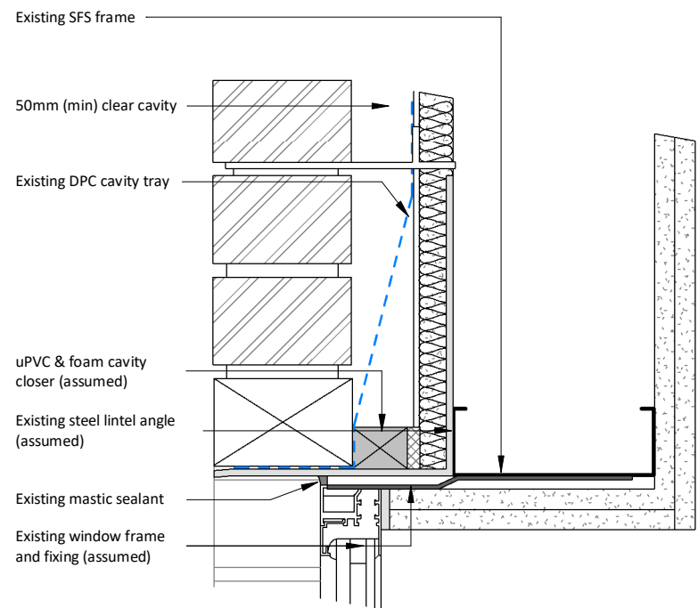
Window Cill as Existing
