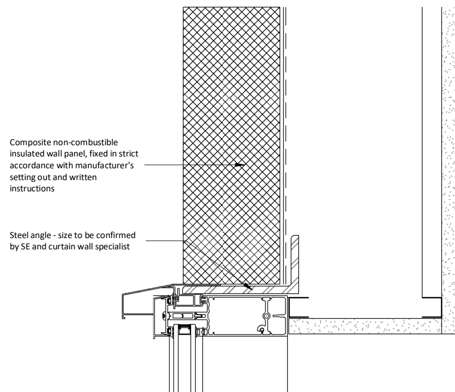
Window Head as Proposed
