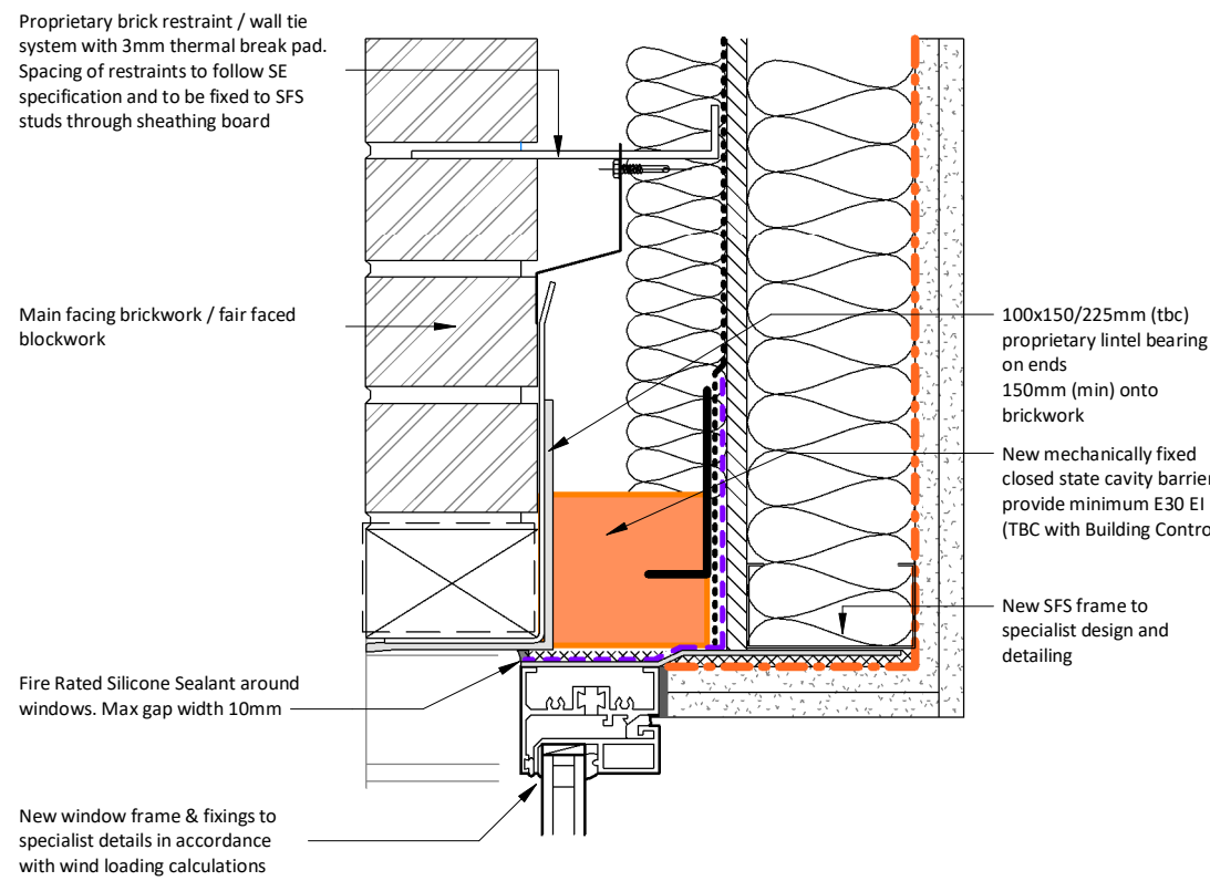
Window Cill as Proposed
