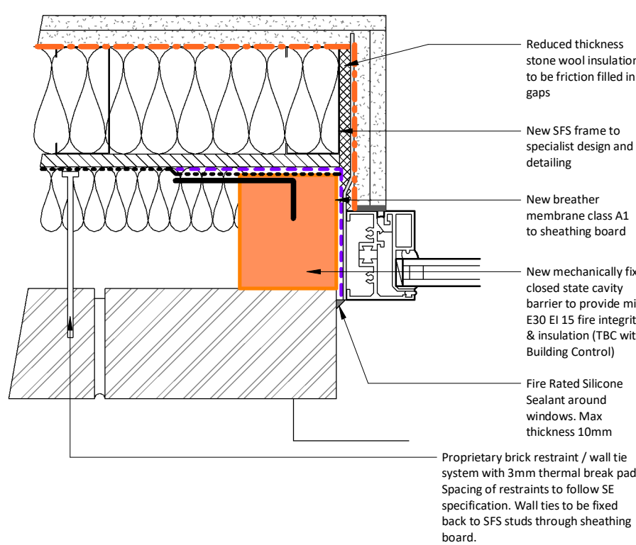
Window Jamb as Proposed
