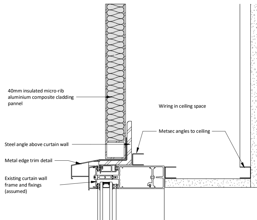
Window Head as Existing
