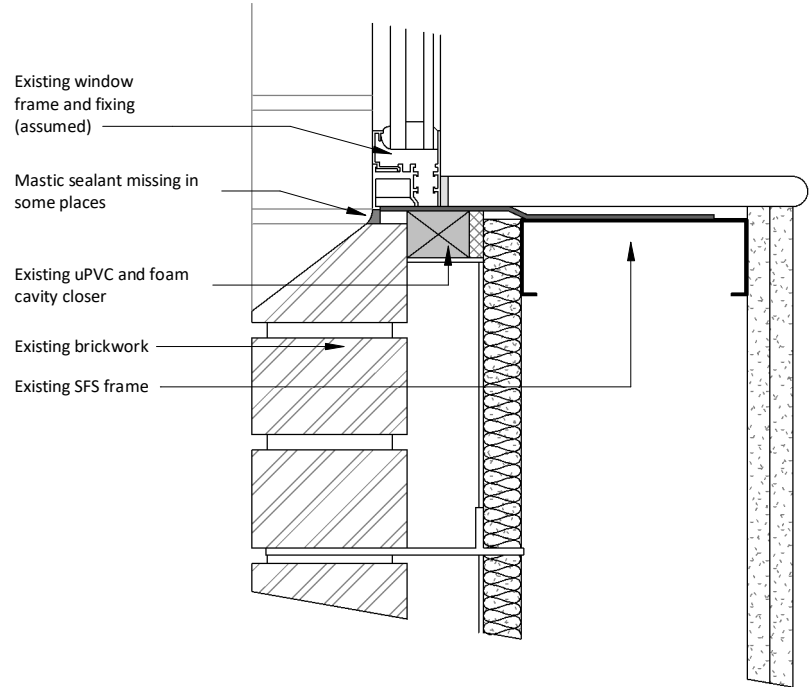
Window Jamb as Existing
