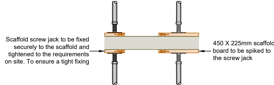
SCREW JACK DETAIL scale 1:25
