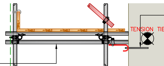
HOOK TIE DETAIL scale 1:25
