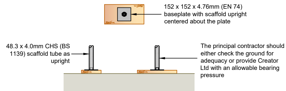
FOUNDATION DETAIL 225 x 38 x 450mm (BS EN 2482) Scaffold Board Solepad Scale — 1:25
