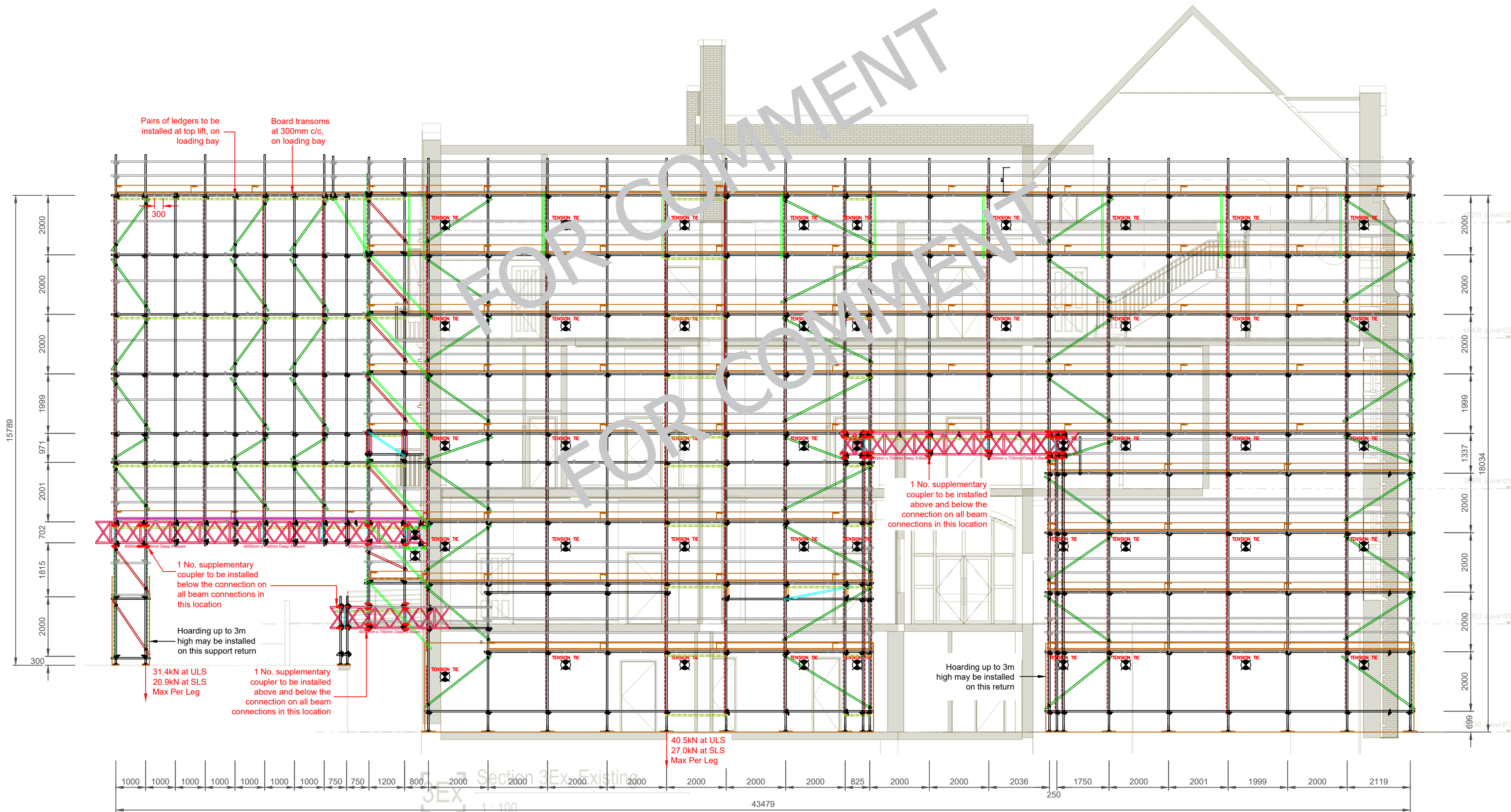
ELEVATION A — A scale 1:100
