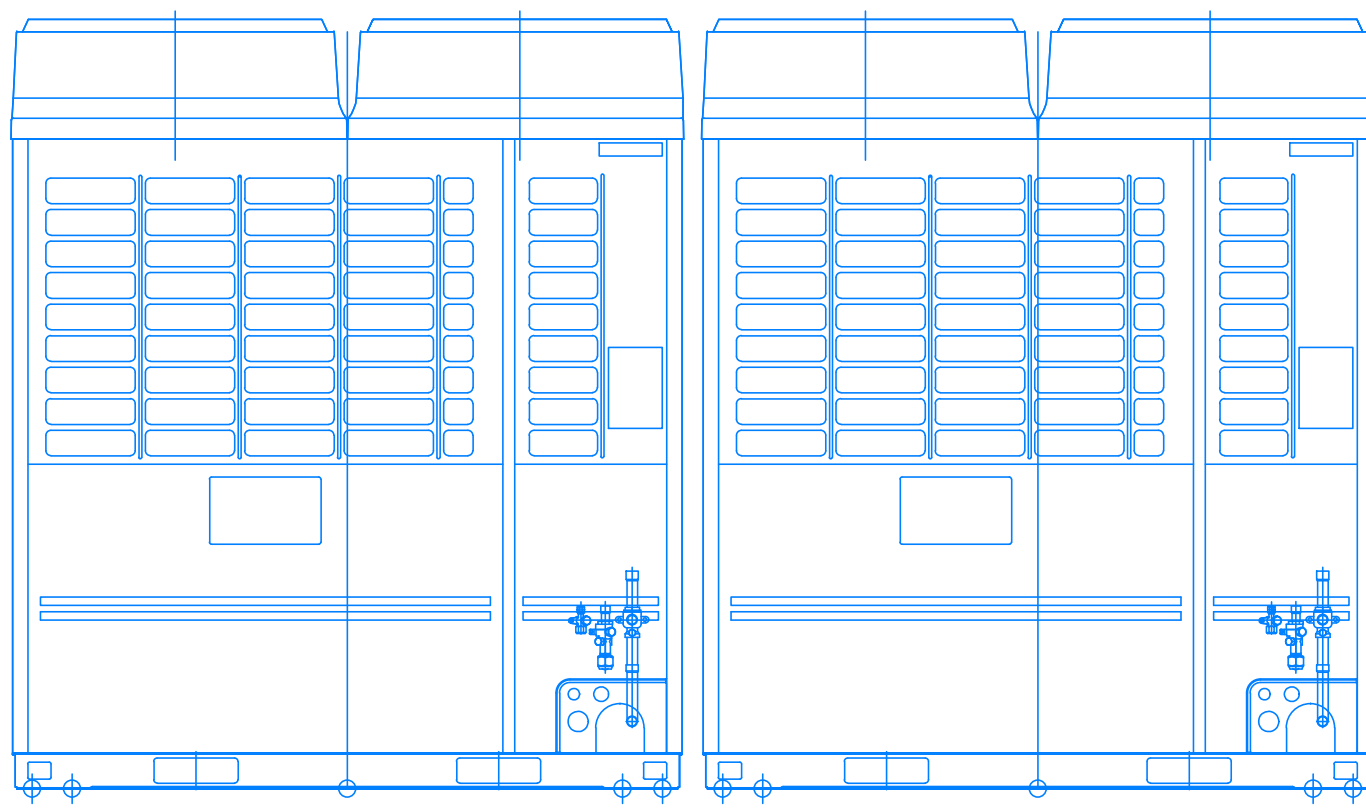
TOSHIBA HEAT PUMP EXTERNAL ROOF CONDENSING UNIT MMY-AP3616FT89-UK - FRONT VIEW (1:25)
