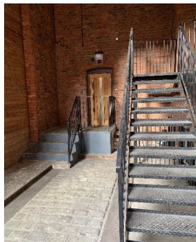
Existing loading bay works under previously approved application 101365/LO/2013/C2. Non-original steel staircase to be removed to accommodate DDA loading bay lift [Photo taken 15.11.19]
