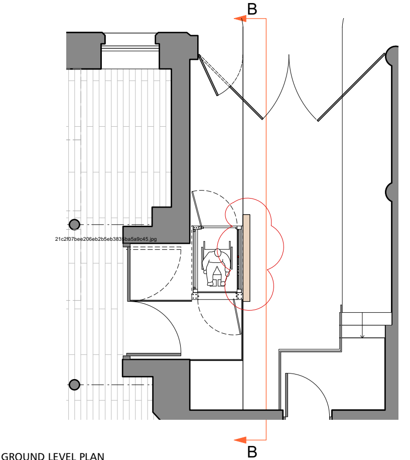
GROUND LEVEL PLAN
