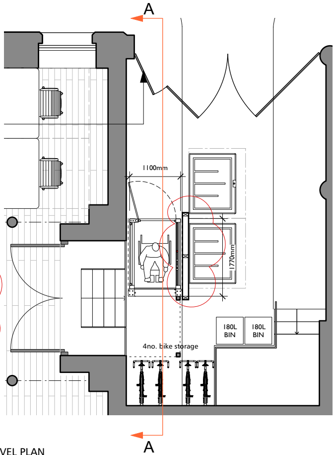
BASEMENT LEVEL PLAN
