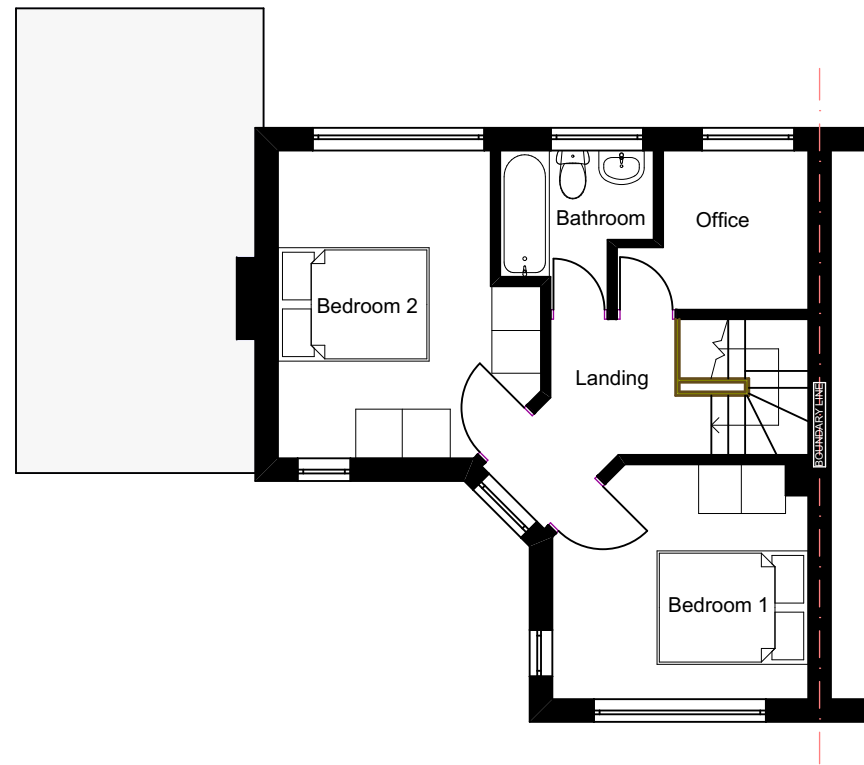
EXISTING GA FIRST FLOOR PLAN
