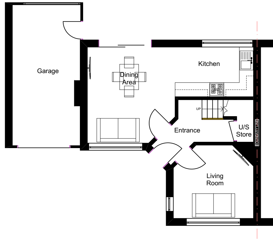
EXISTING GA GROUND FLOOR PLAN
