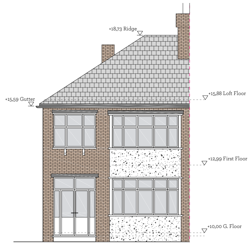
Front Elevation - no change
