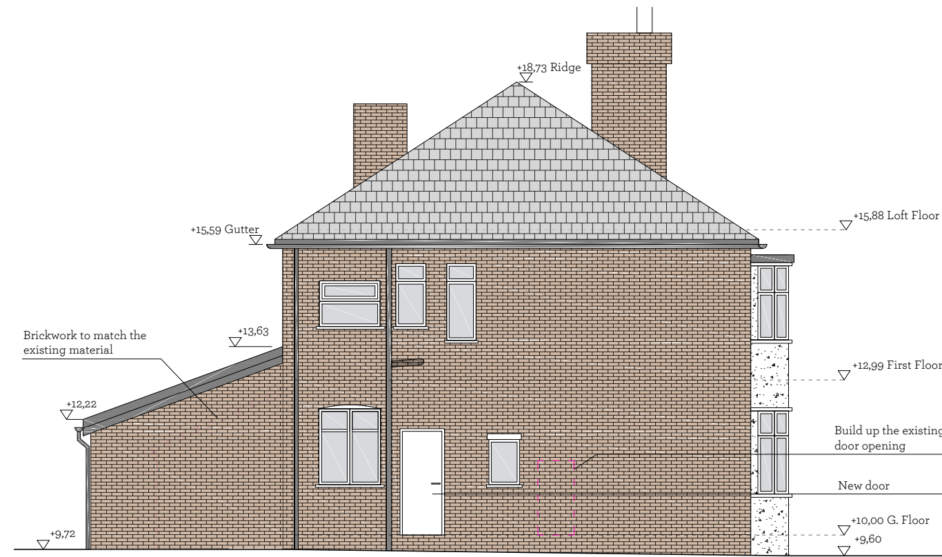
Side Elevation
