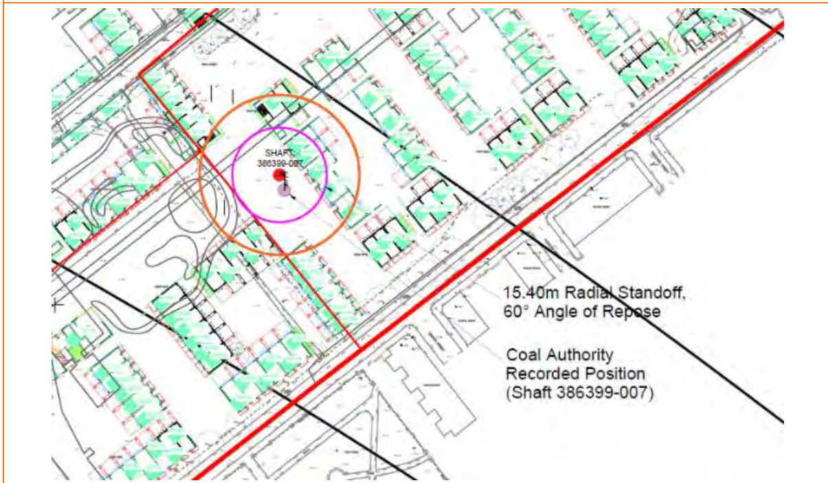
FIGURE 2.1 – MAXIMUM EXTENT OF RADIAL INFLUENCE – SHAFT COLLAPSE.
