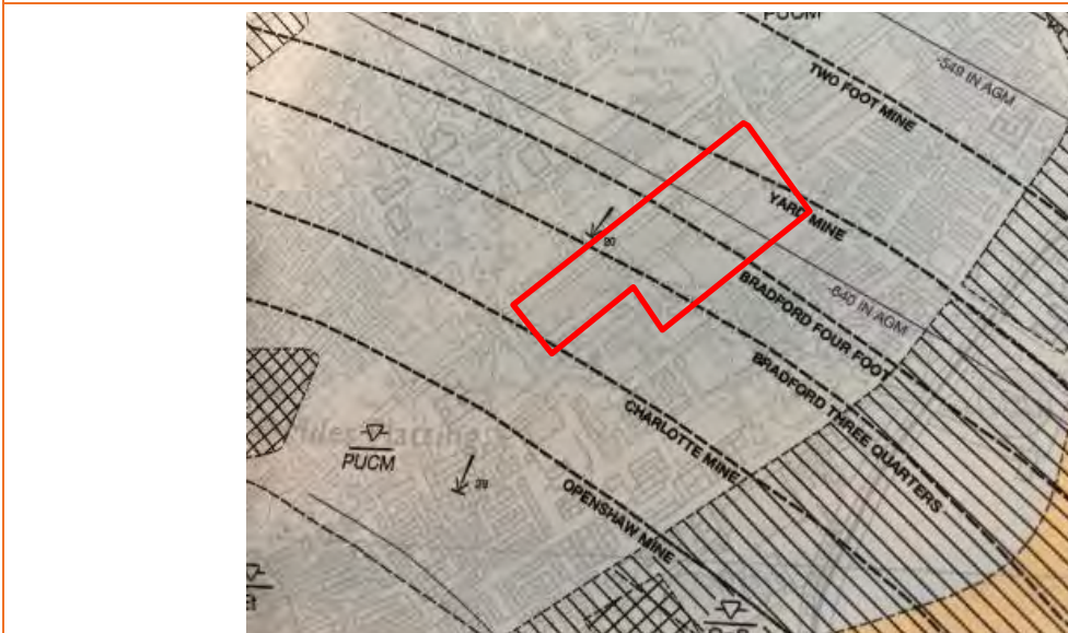
FIGURE 2.4 – EXTRACT OF 1:10,000 BGS MAPPING
