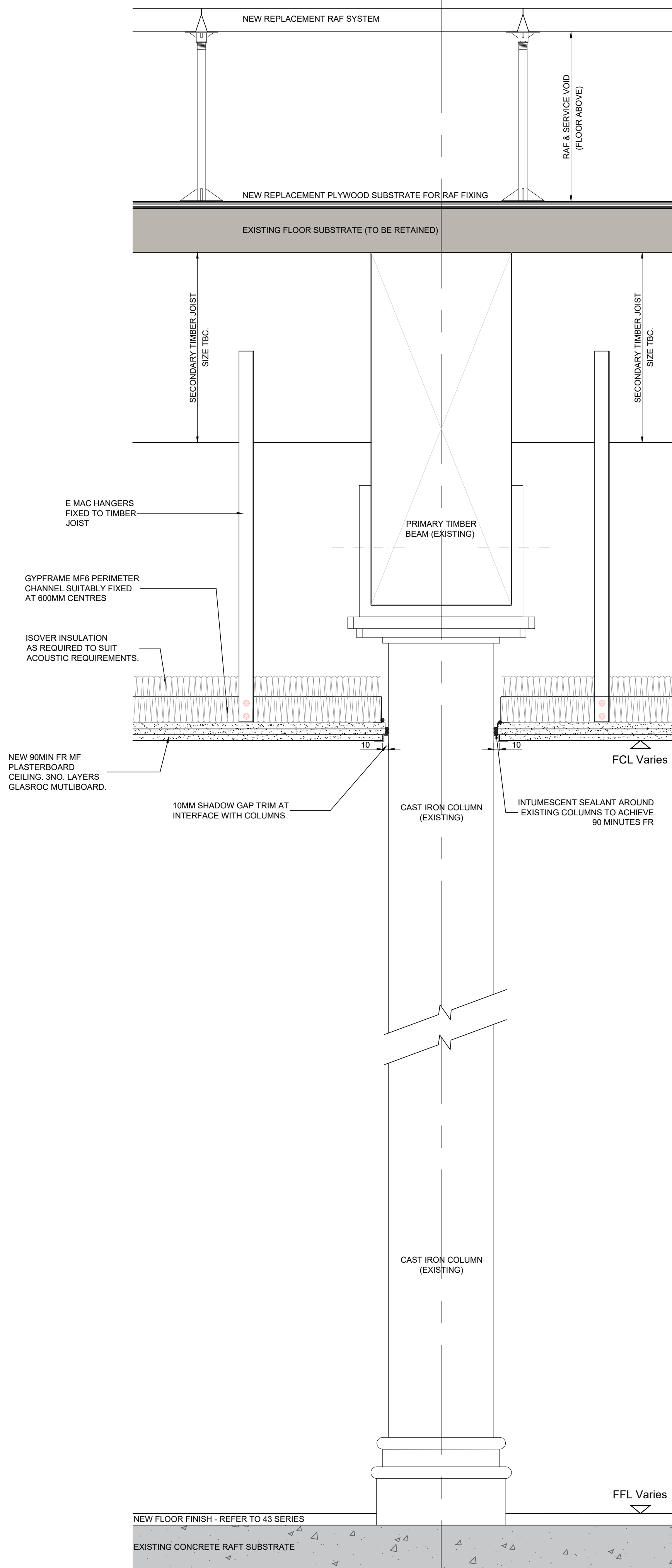
BASEMENT - NEW 90MIN FR CEILING TYPICAL DETAIL: JUNCTION WITH EXISTING COLUMN
