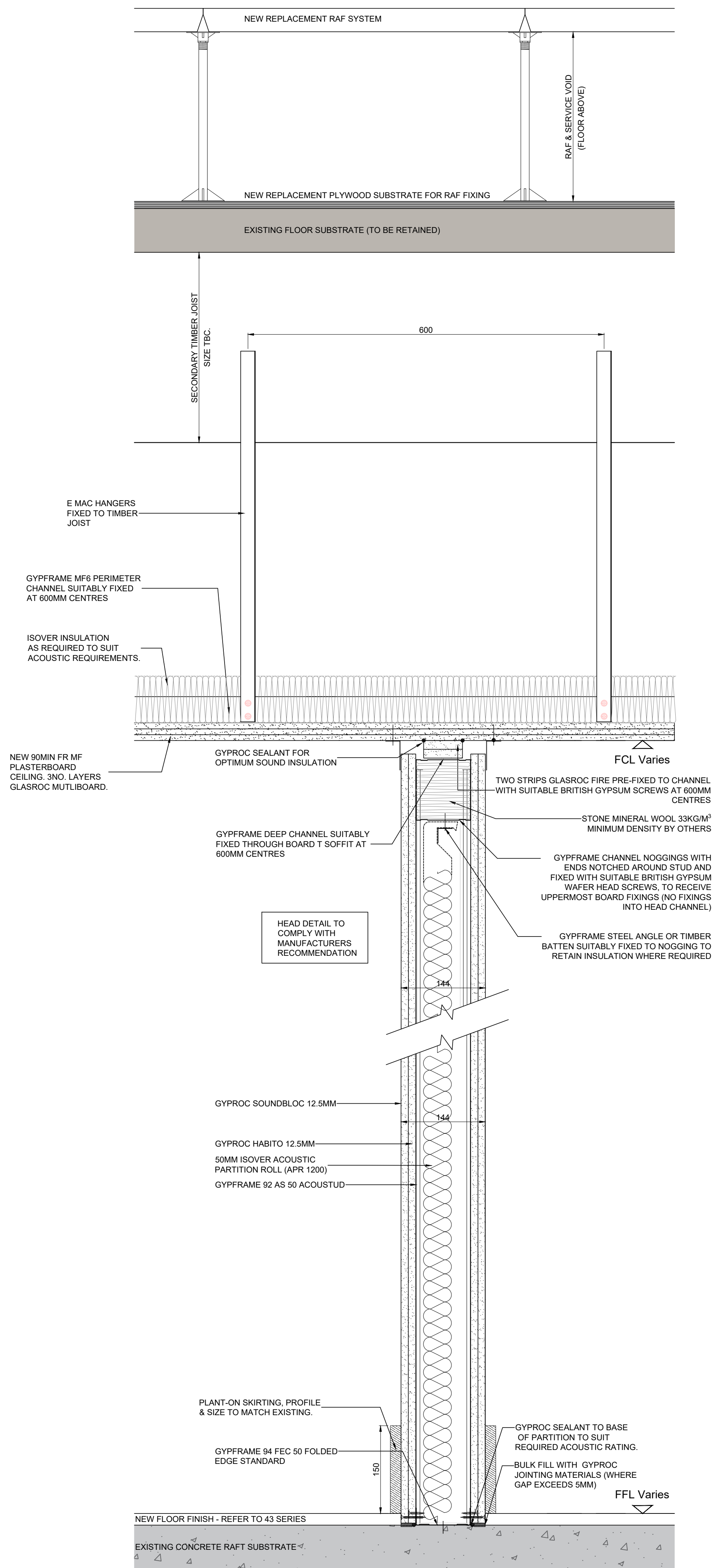
BASEMENT - NEW 90MIN FR CEILING TYPICAL DETAIL: JUNCTION WITH NEW 90MIN FR PARTITION
