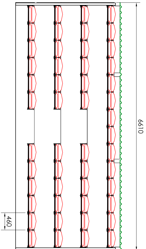
PLAN VIEW (WITHOUT ROOF)
