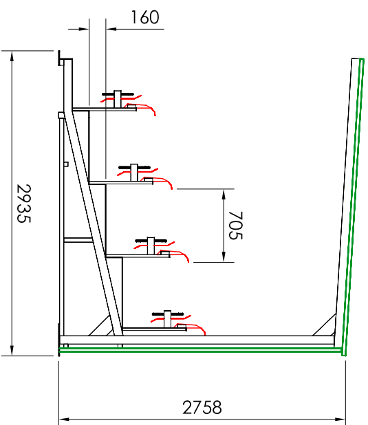
TYPICAL SECTION
