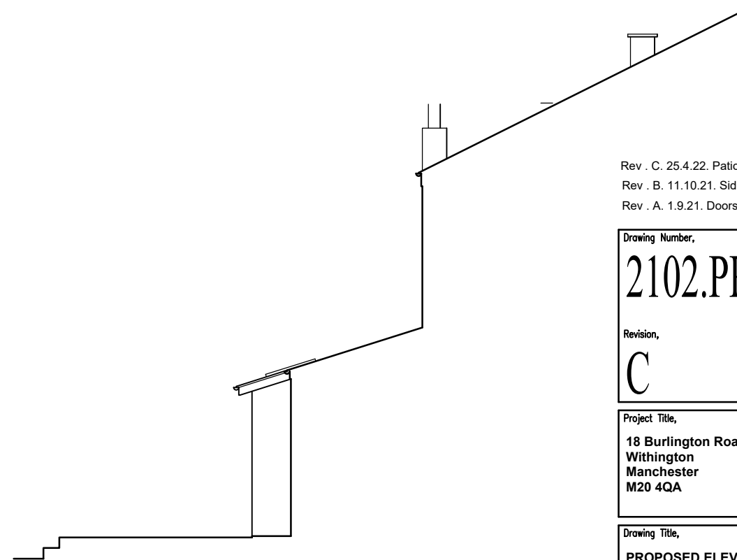
PROPOSED SIDE ELEVATION / SECTION
