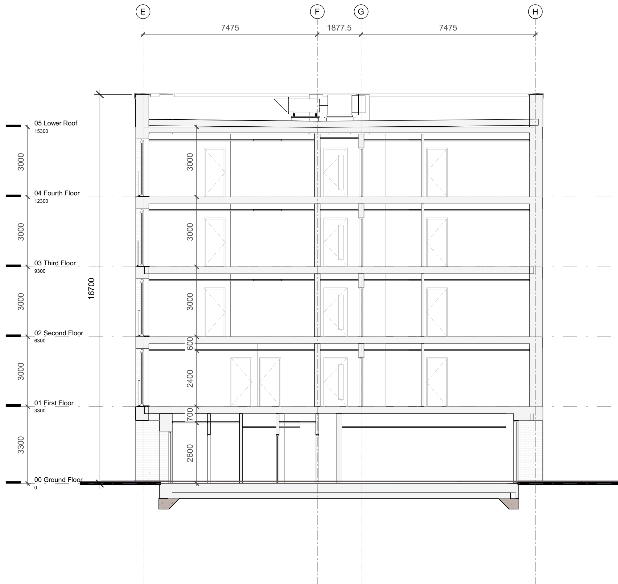
Section AA
