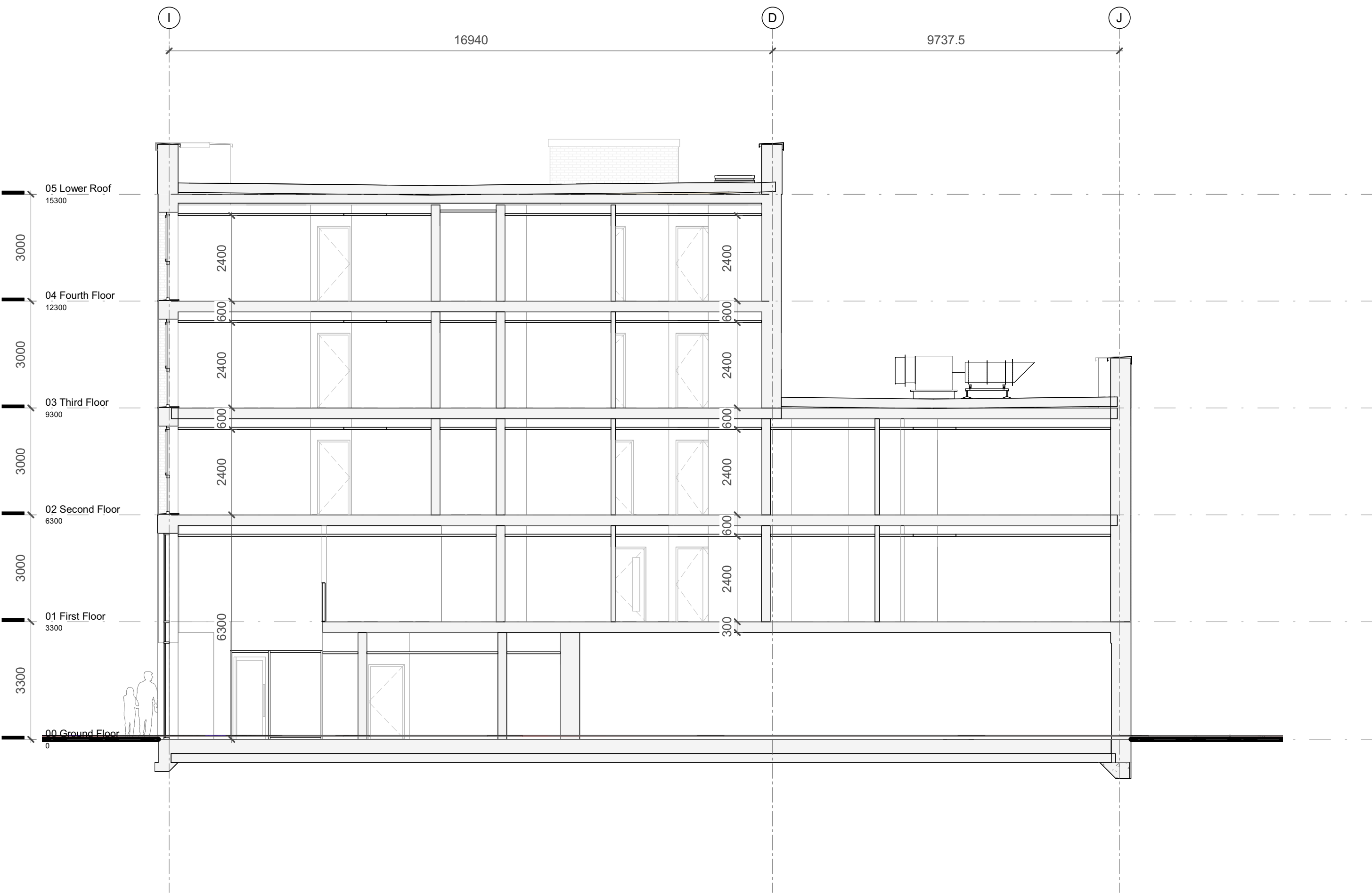
Section BB
