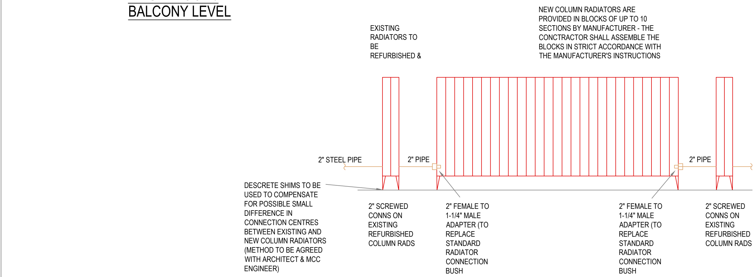
BALCONY RADIATOR PIPING (NTS)
