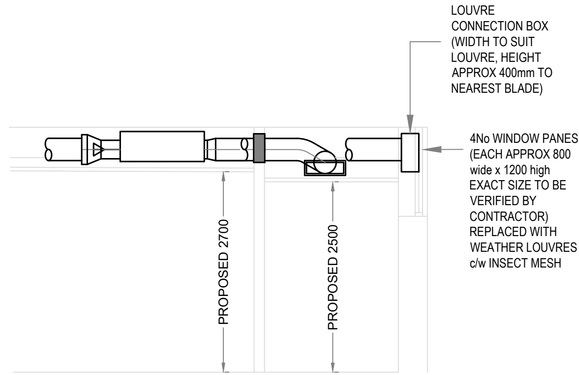
SECTION A-A Approx 1:50
