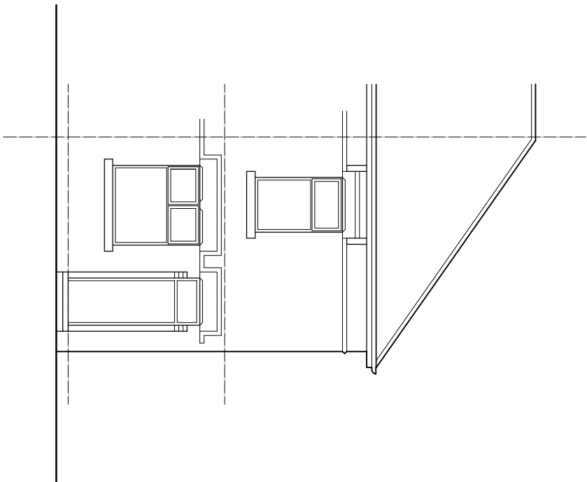
FRONT ELEVATION 1:100
