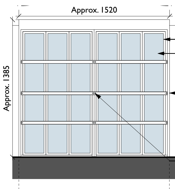
Proposed Elevation Scale: 1:20
