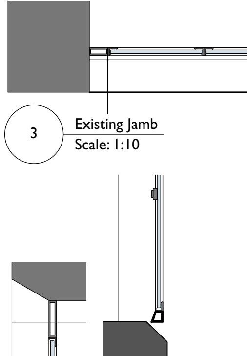
Existing Head and Cill Scale: 1:10
