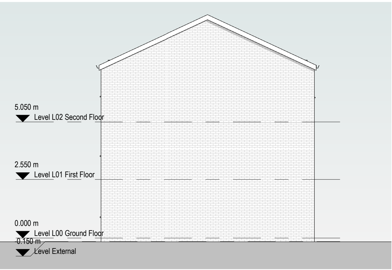
2 Existing West Elevation 1 : 100
