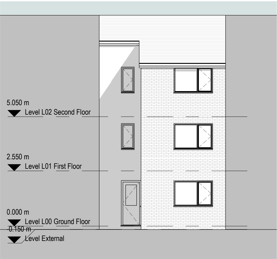
3 Existing North Elevation 1 : 100
