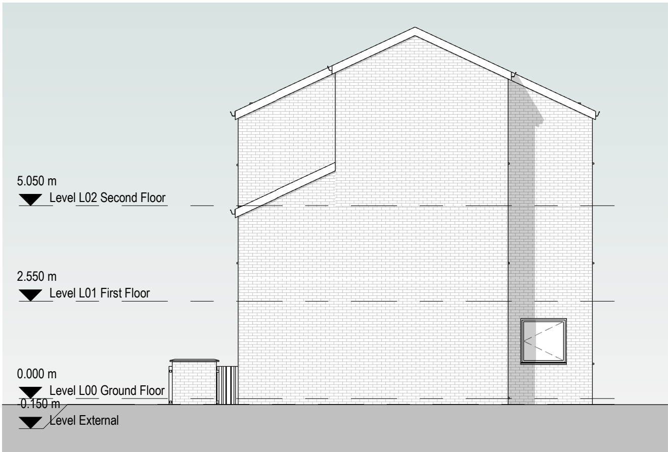
4 Existing East Elevation 1 : 100
