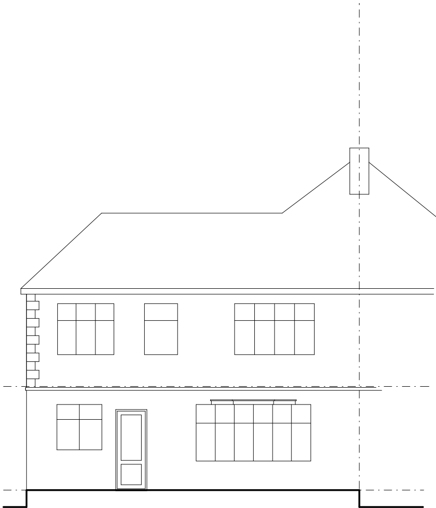
Rear Elevation
