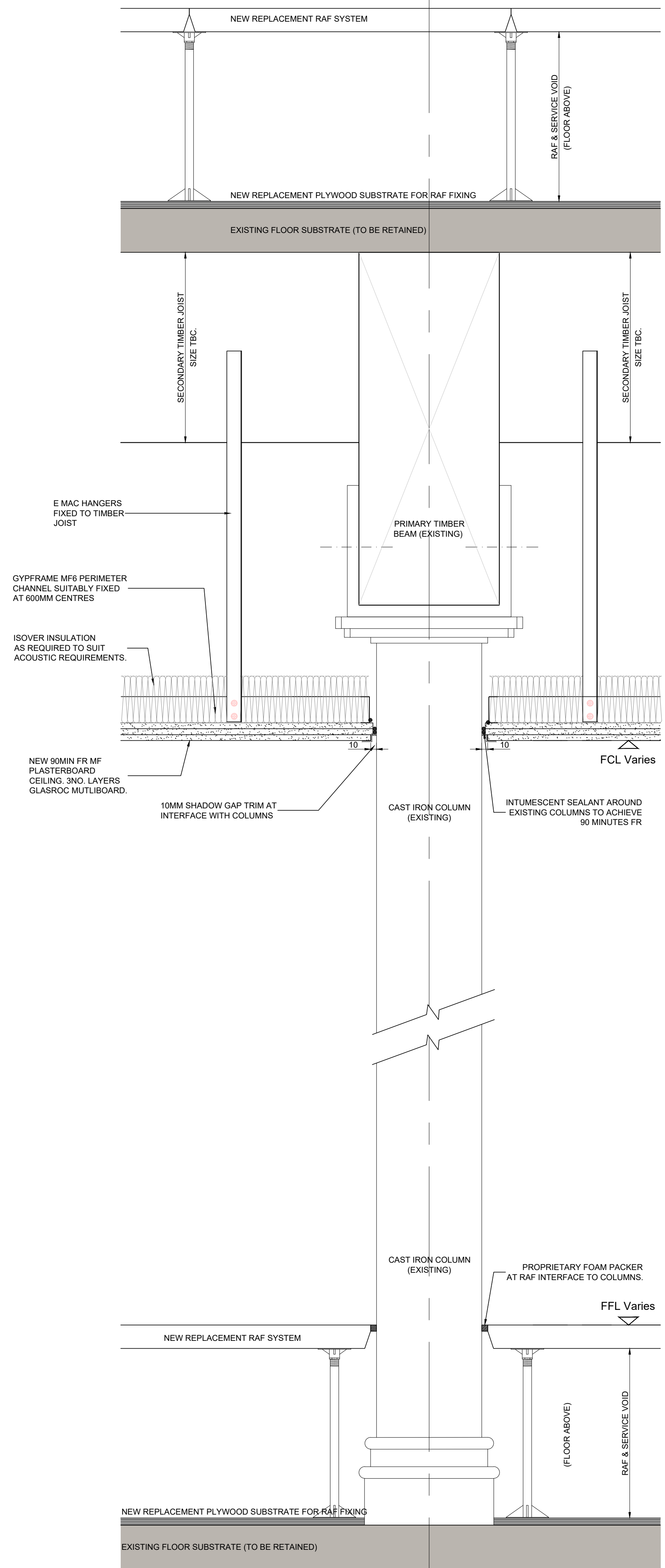
LOWER GROUND FLOOR - NEW 90MIN FR CEILING TYPICAL DETAIL: JUNCTION WITH EXISTING COLUMN
