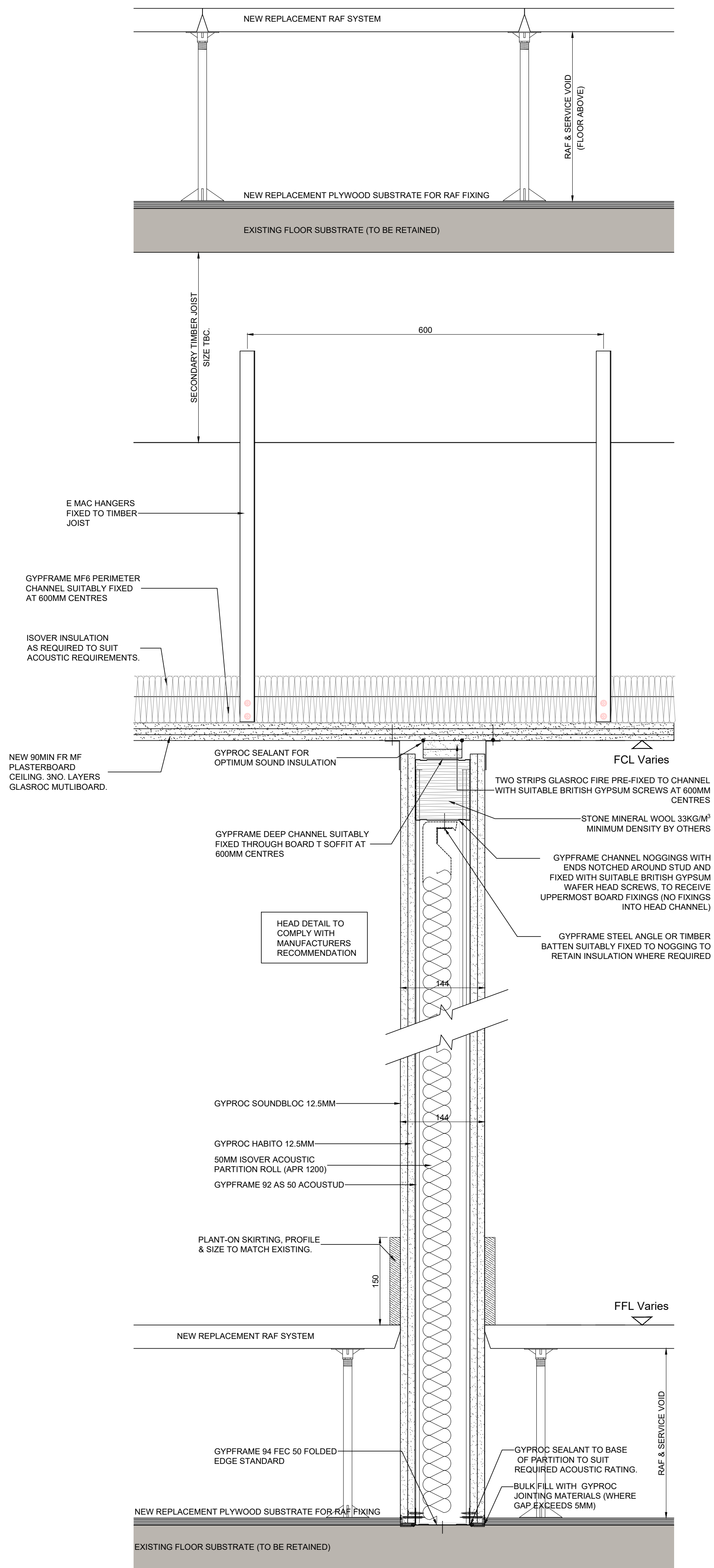
LOWER GROUND FLOOR - NEW 90MIN FR CEILING TYPICAL DETAIL: JUNCTION WITH NEW 90MIN FR PARTITION
