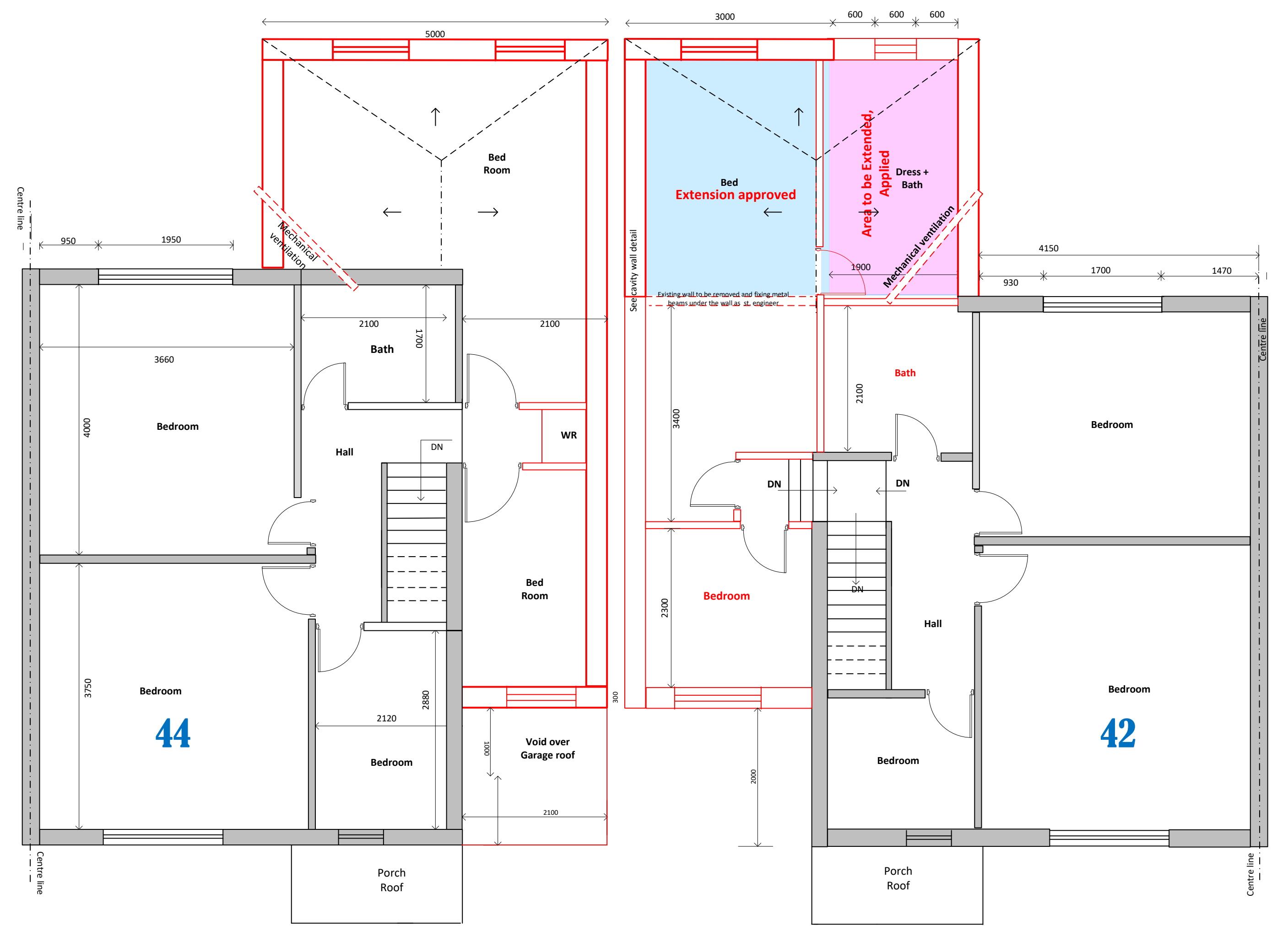
DRAWING NO :6 Scale 1 = 50
