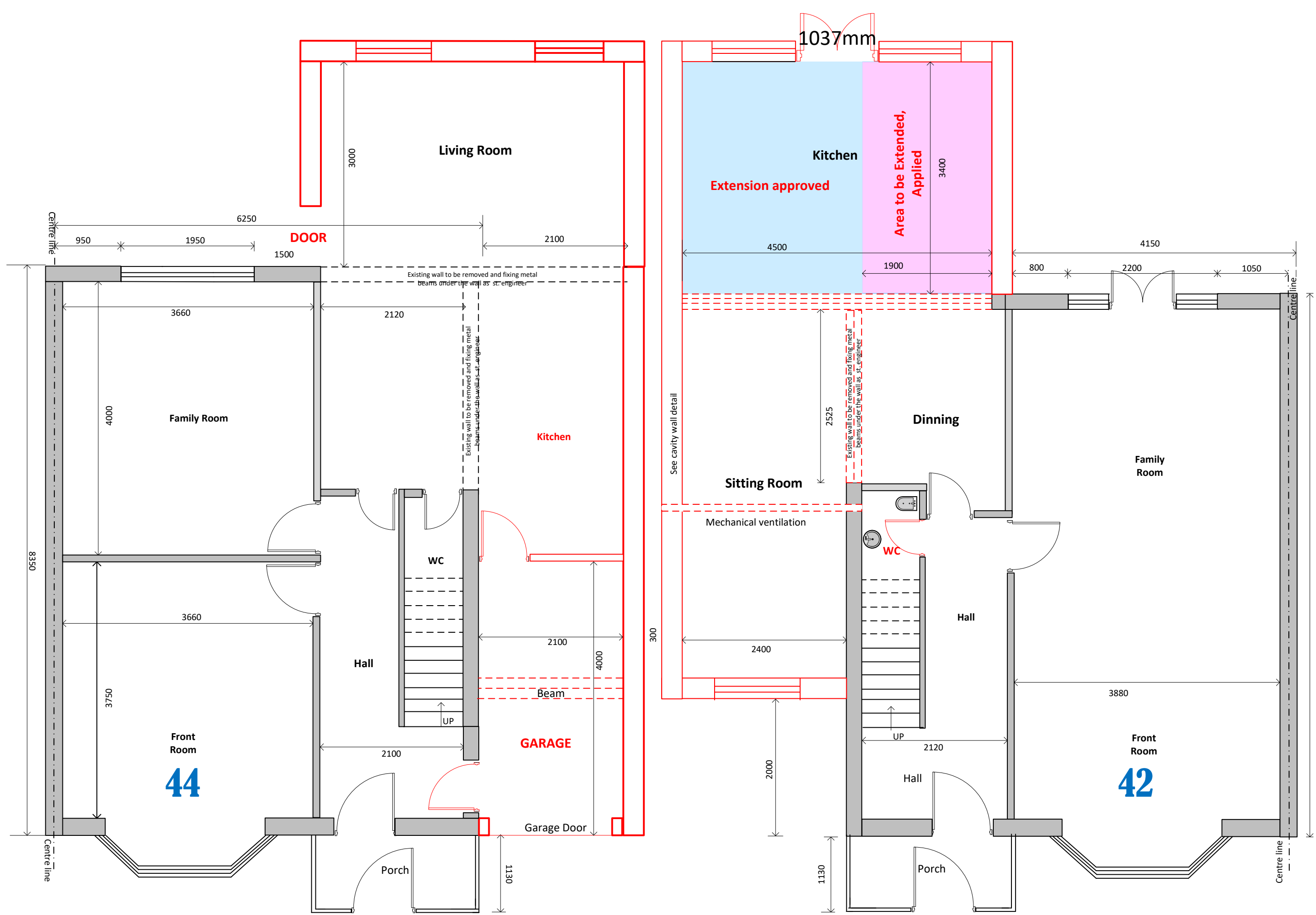
DRAWING NO: 5 Scale 1 = 50
