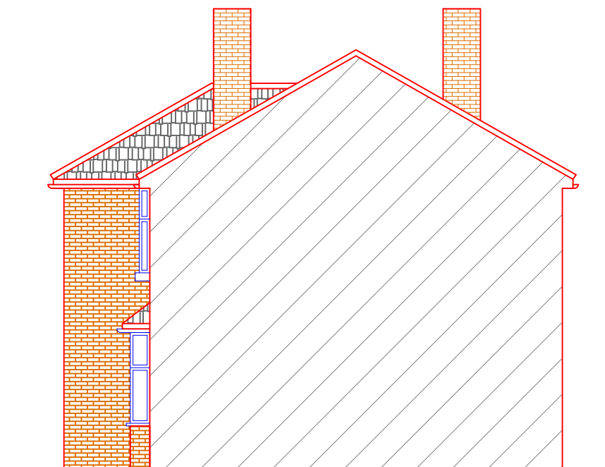
PROPOSED SIDE ELEVATION - B
