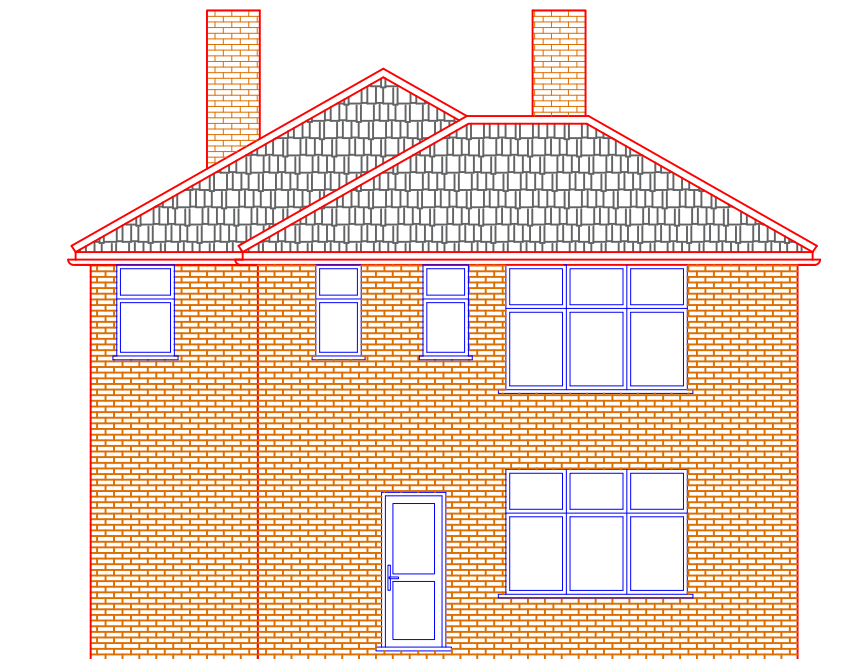
PROPOSED SIDE ELEVATION - A
