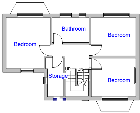
2 Existing First Floor 1 : 150
