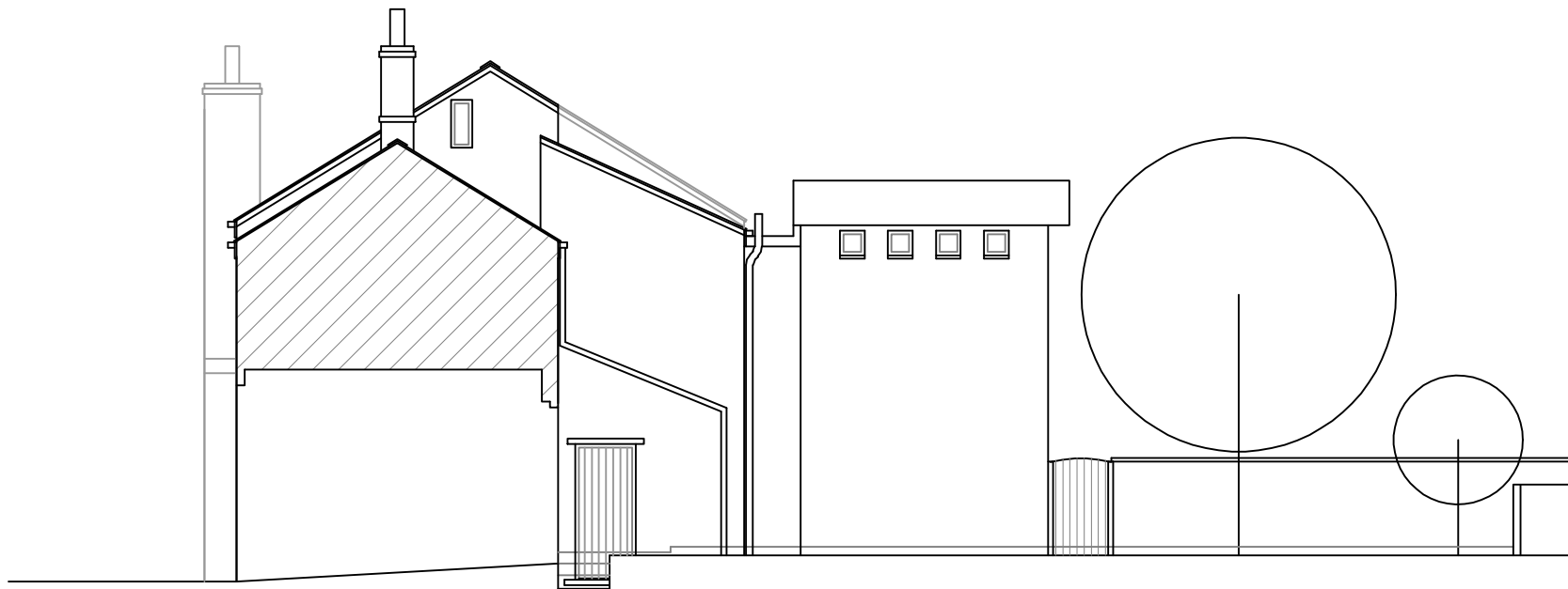
133 NELL LANE GINNEL SECTION (BEHIND FENCE) - EXISTING
