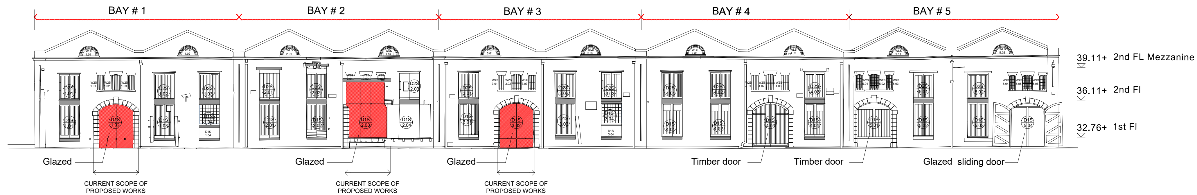
DATUM 25m SOUTH EXTERNAL ELEVATION
