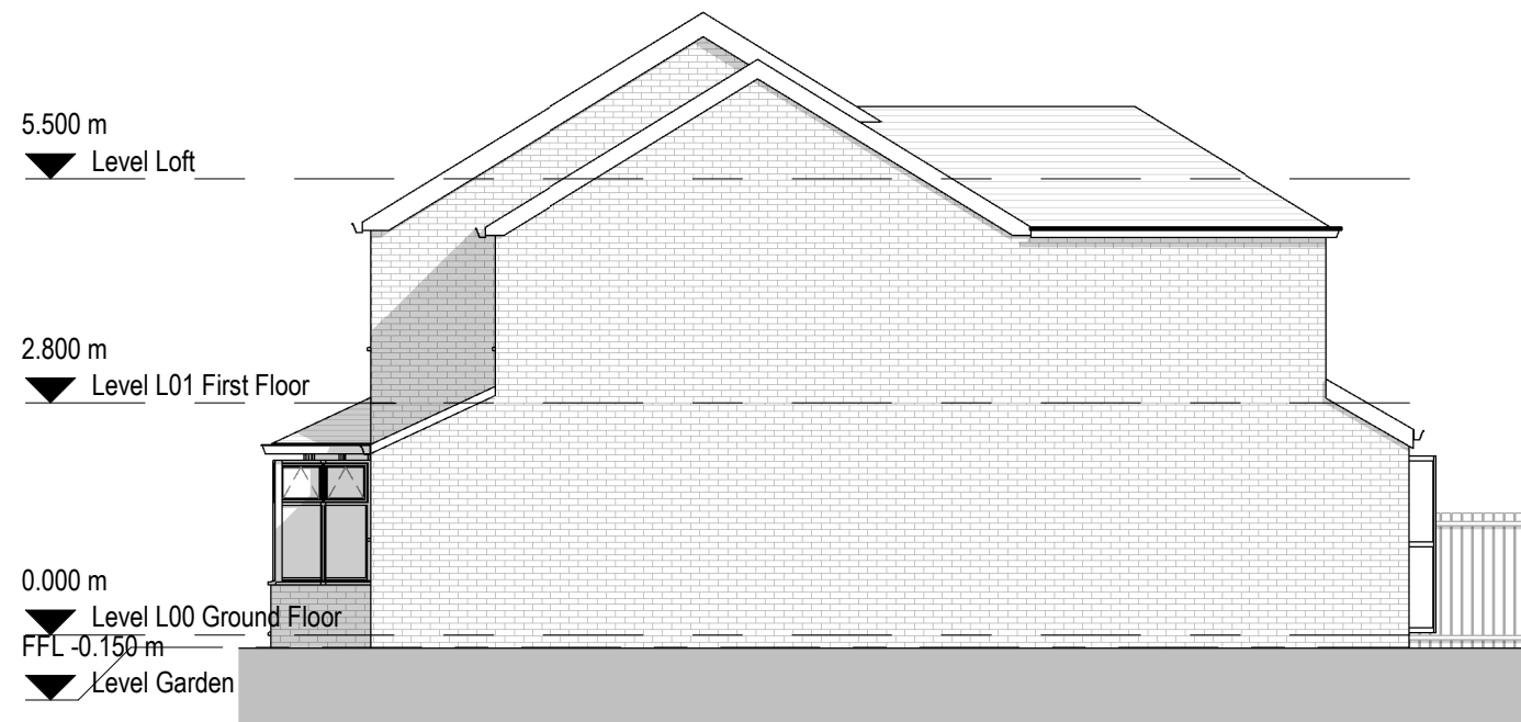
1 Proposed West Elevation 1 : 100
