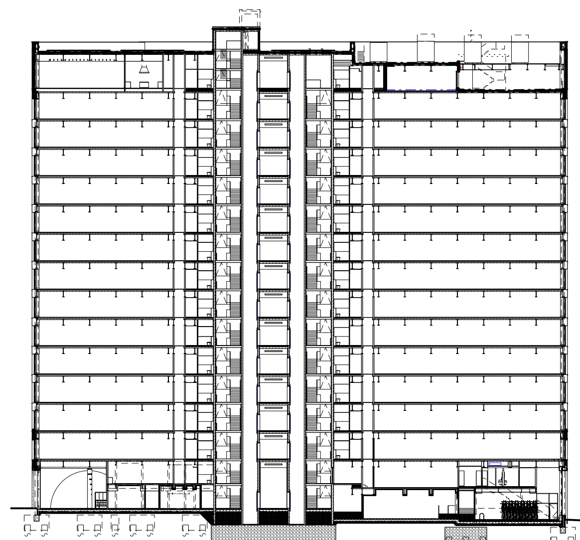
PROPOSED SECTION F-F (1:500)
