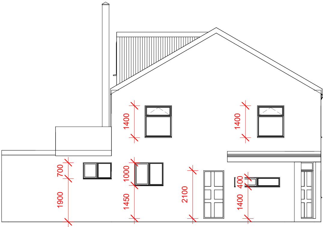
3 proposed, front elevation, setout 1 : 100
