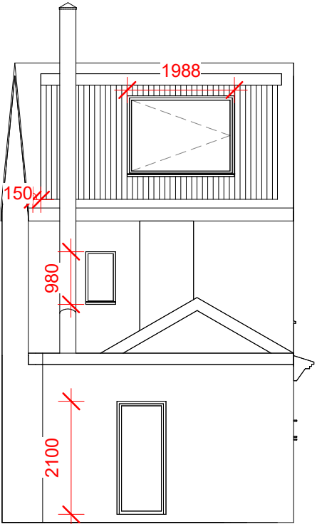
2 proposed, right elevation, setout 1 : 100
