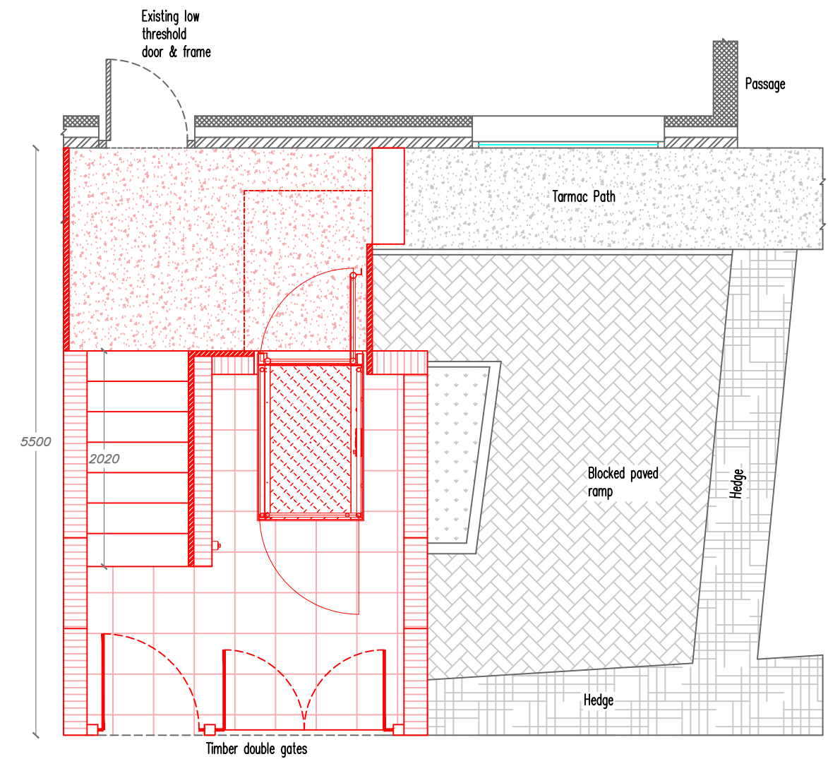
Proposed layout
