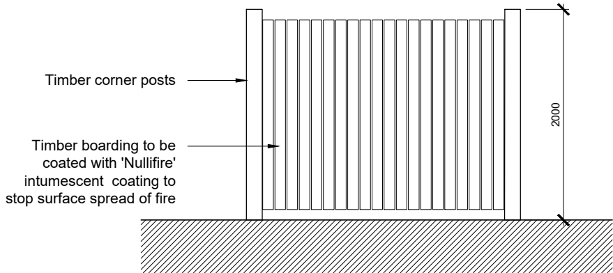
Rear Elevation
