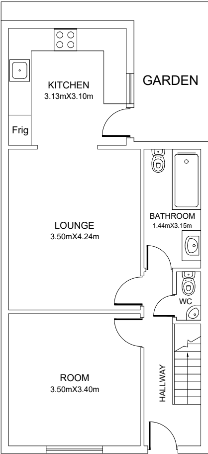
PROPOSED GROUND FLOOR
