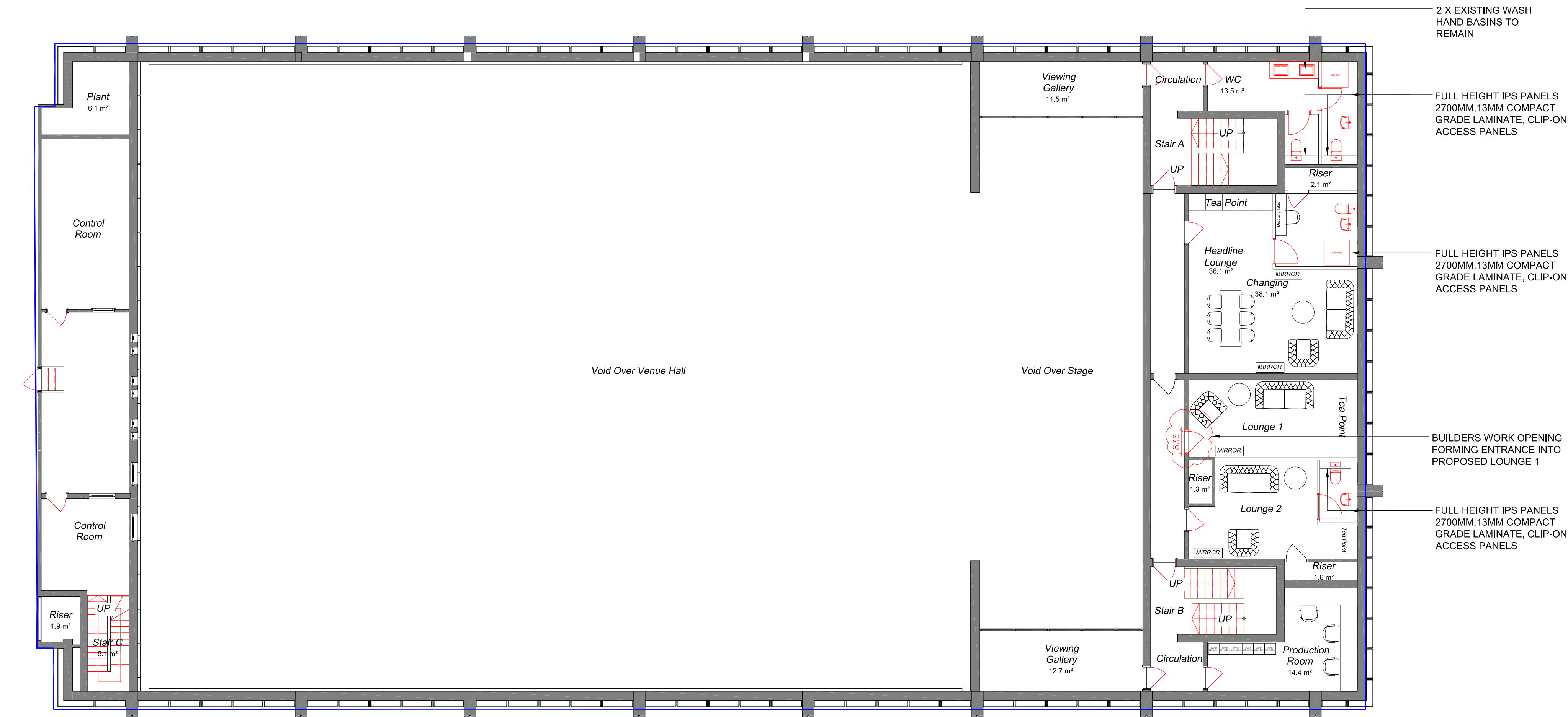
01 MEZZANINE GENERAL ARRANGEMENT PLAN Scale 1:100
