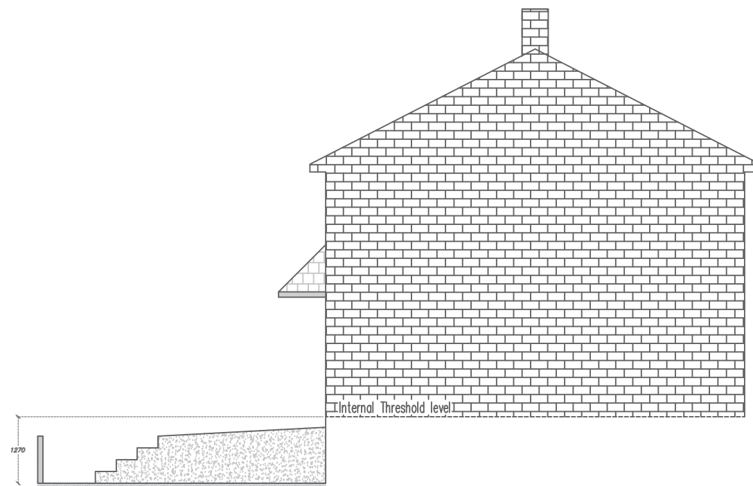
Existing Right hand side elevation
