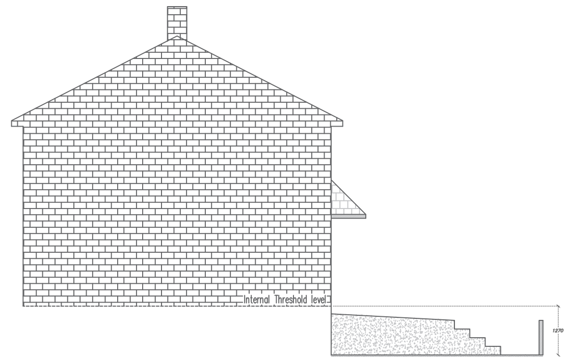
Existing Left hand side elevation
