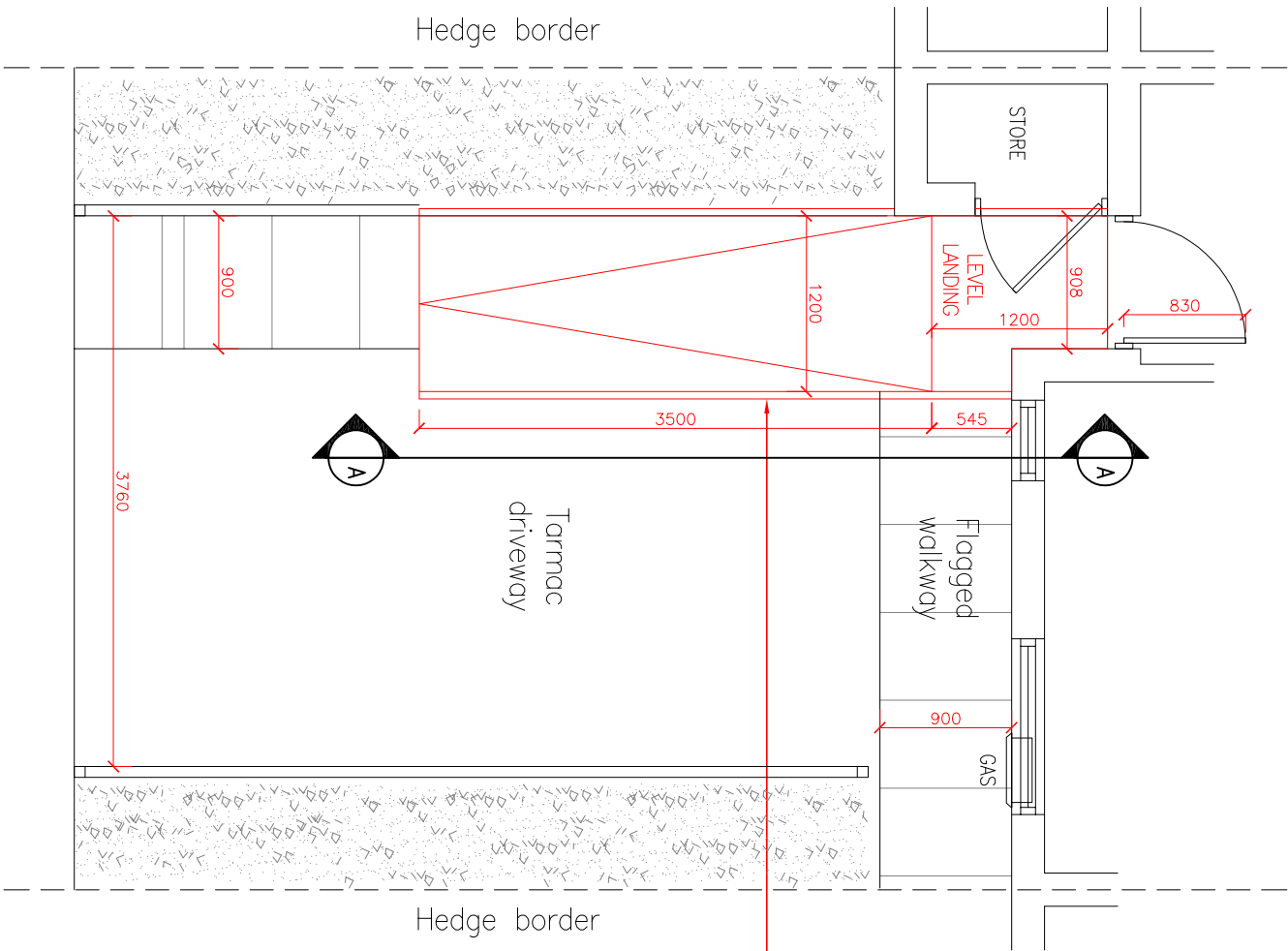
PROPOSED FRONT GARDEN LAYOUT
