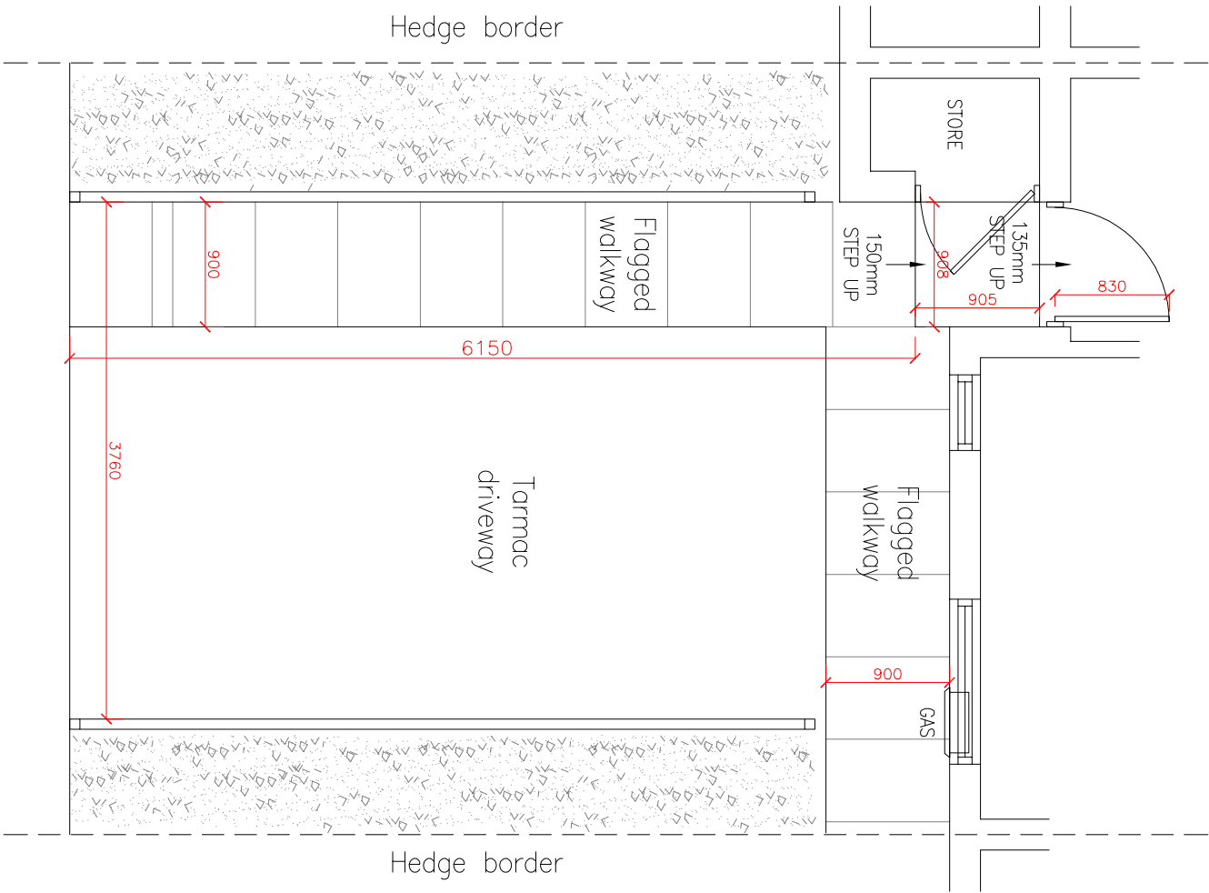
EXISTING FRONT GARDEN LAYOUT
