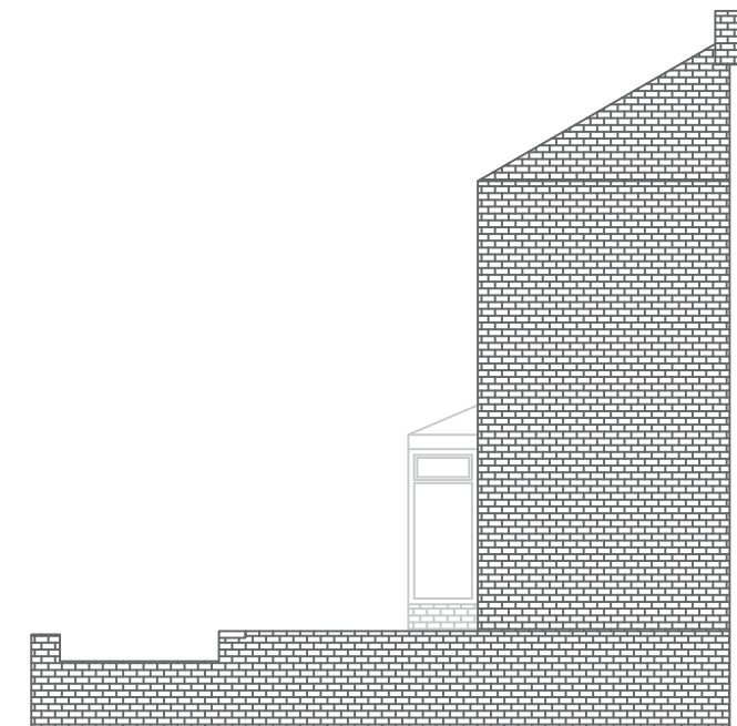
Existing RHS Elevation
