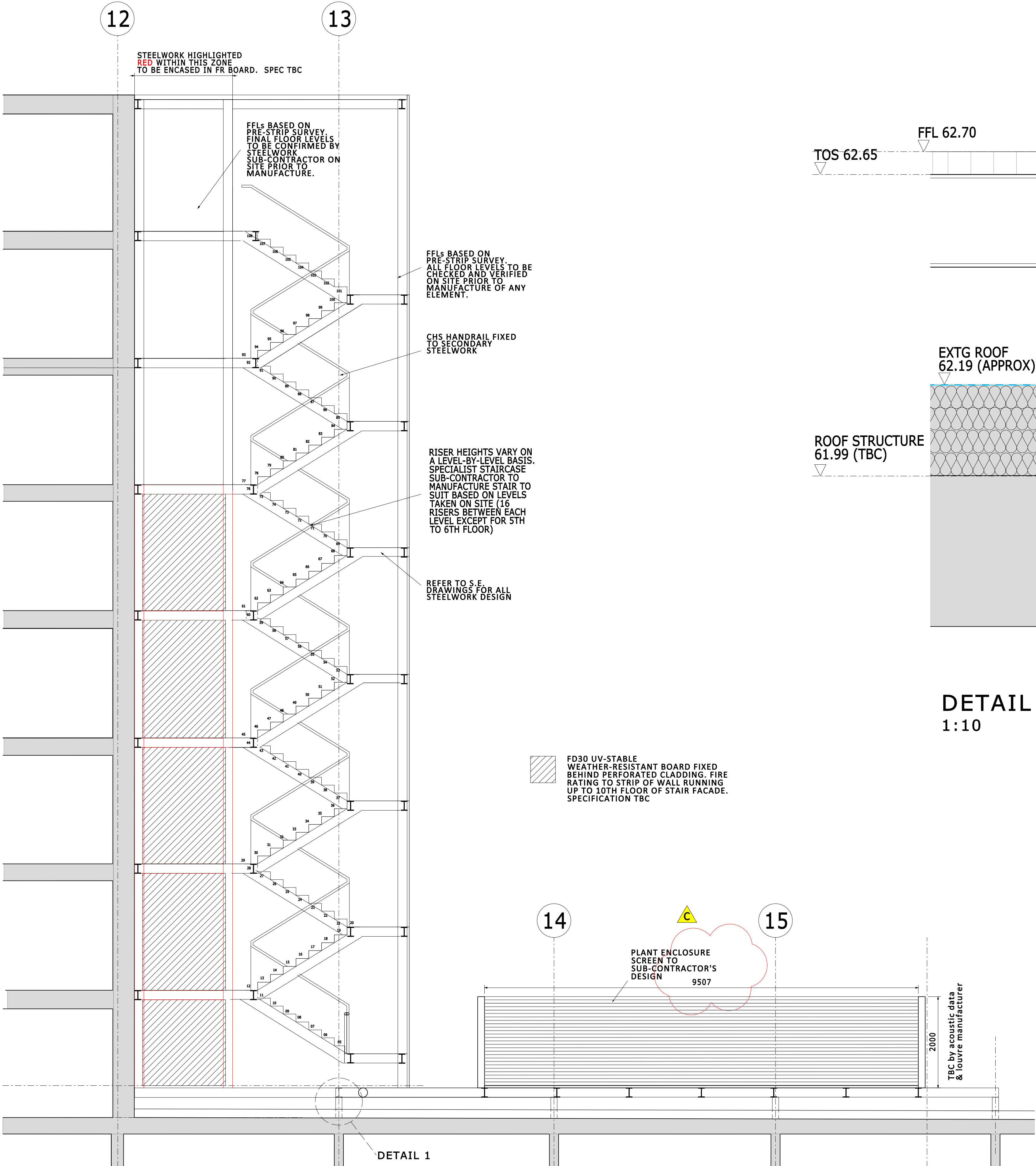
SECTION CC 1:50
