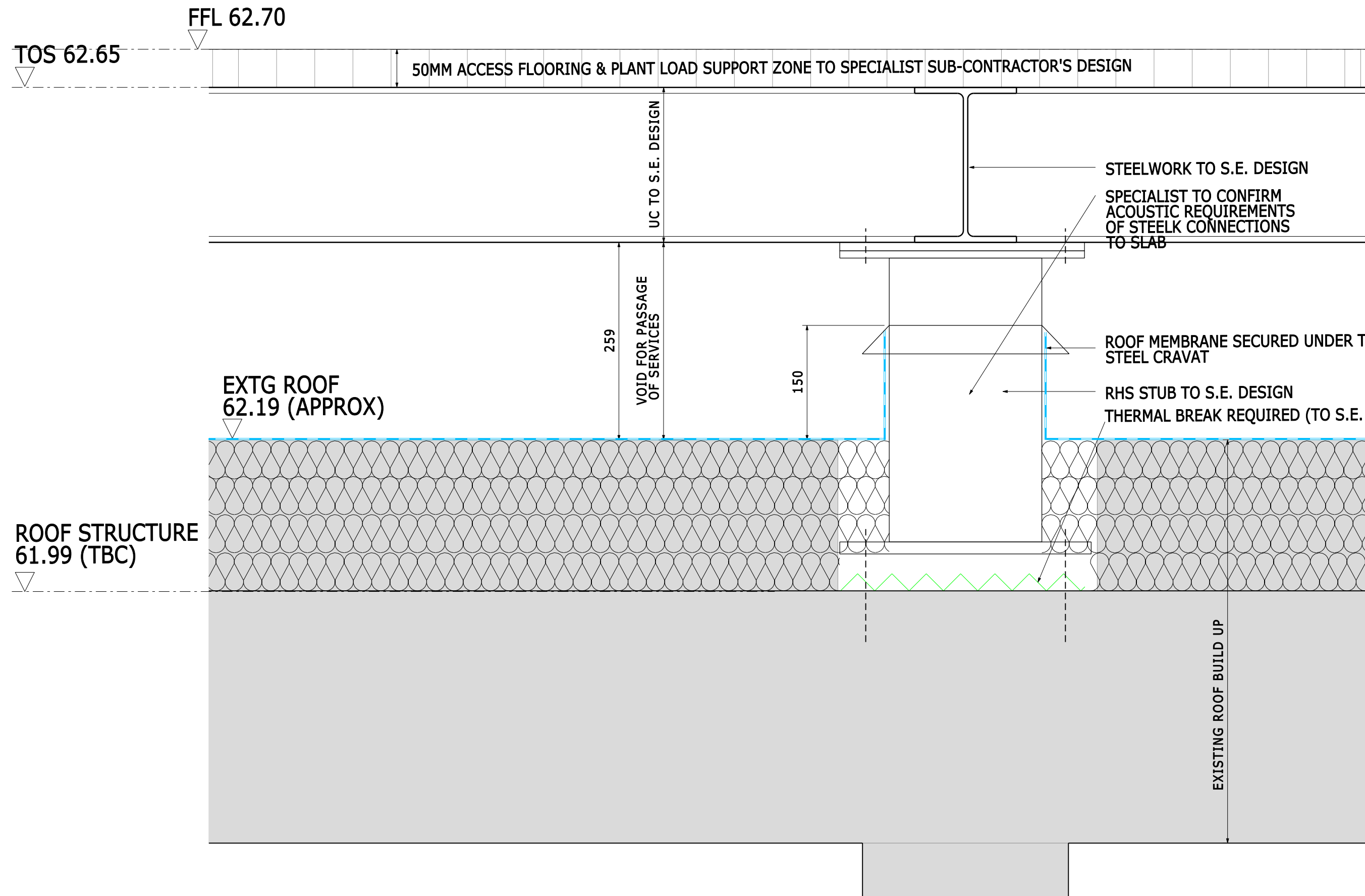
DETAIL 1 1:10
