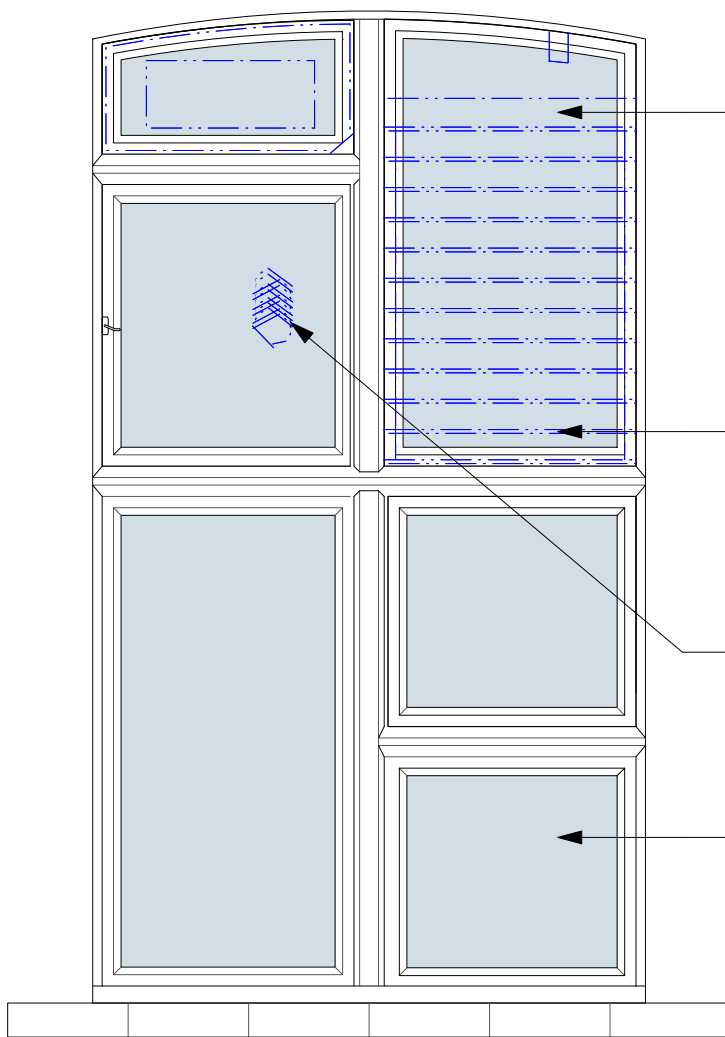
4 Proposed Window Elevation Scale: 1:20
