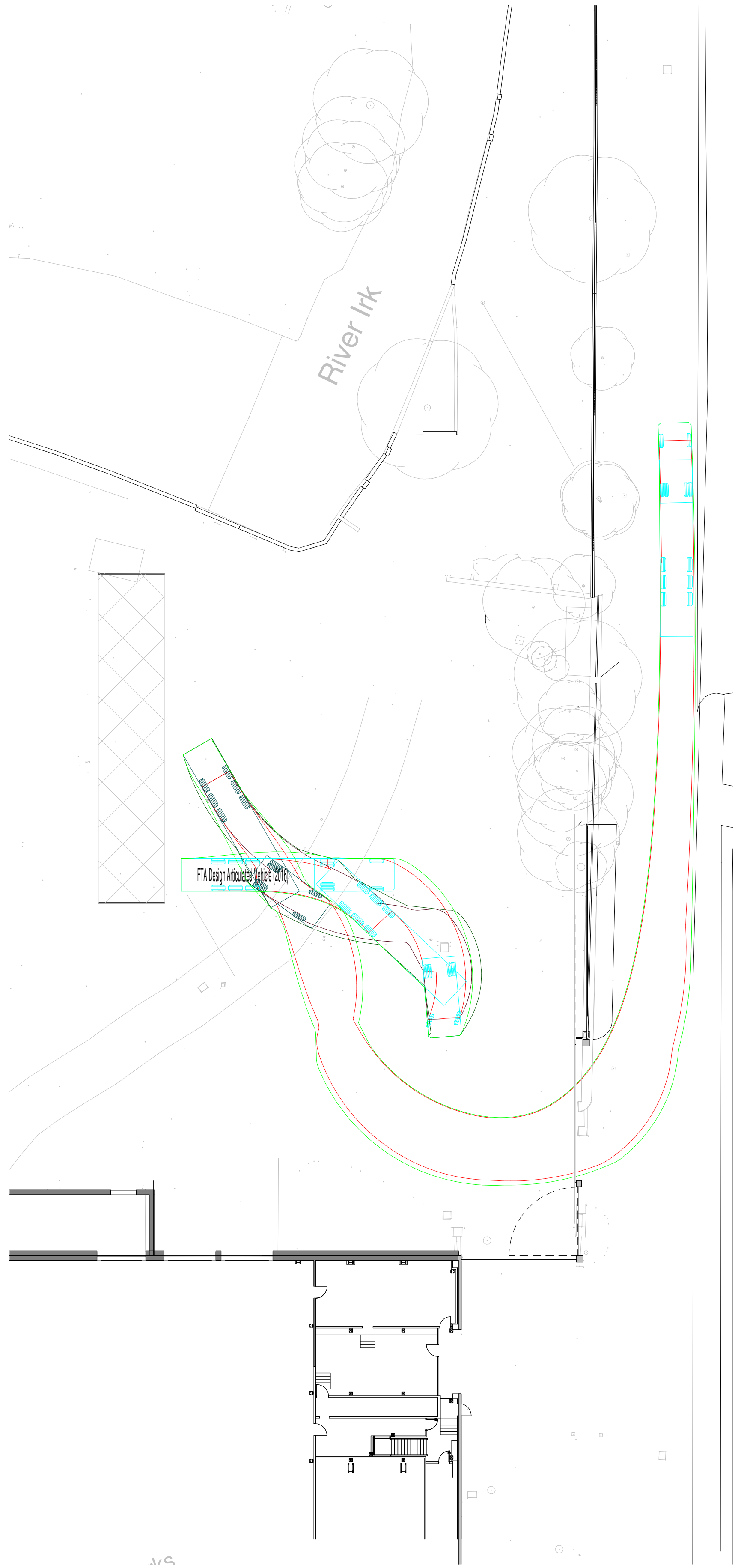
2 HGV Vehicle Tracking Exit 1 : 250
