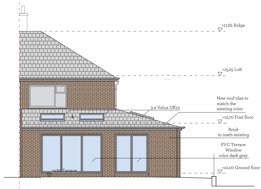
Garden Elevation
