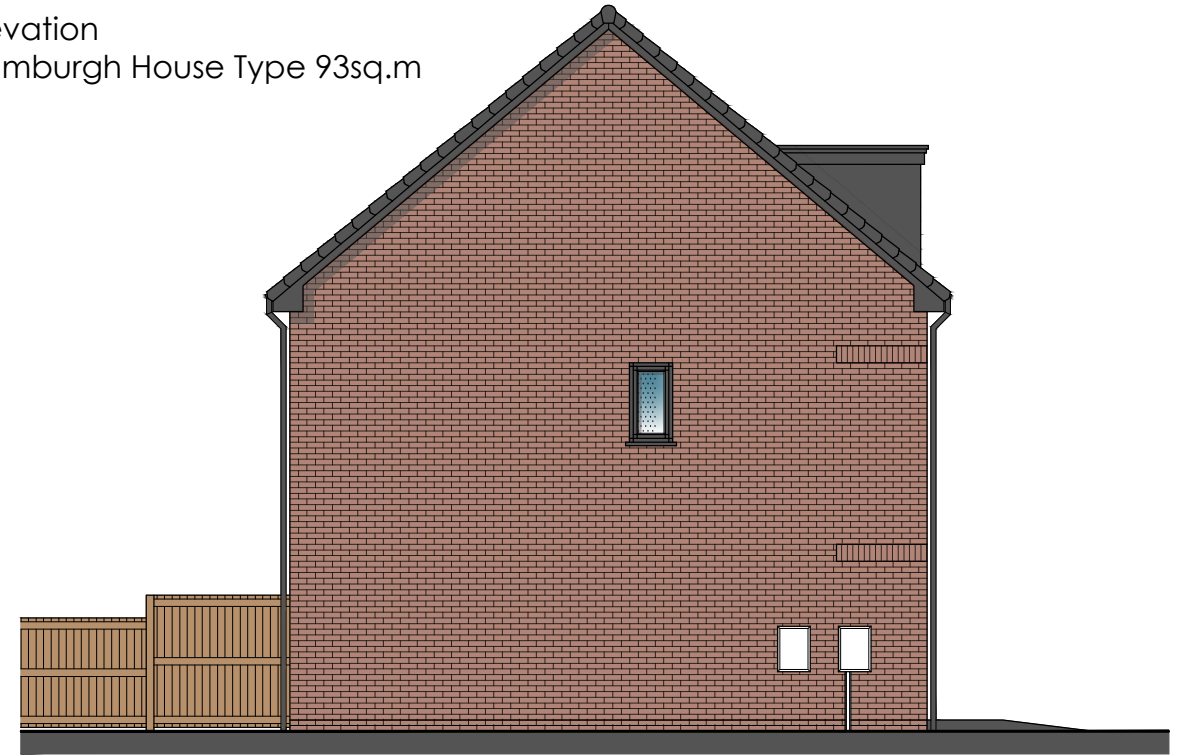
Side Elevation 3B4P Bamburgh House Type 93sq.m (Adjoining Property Handed)
