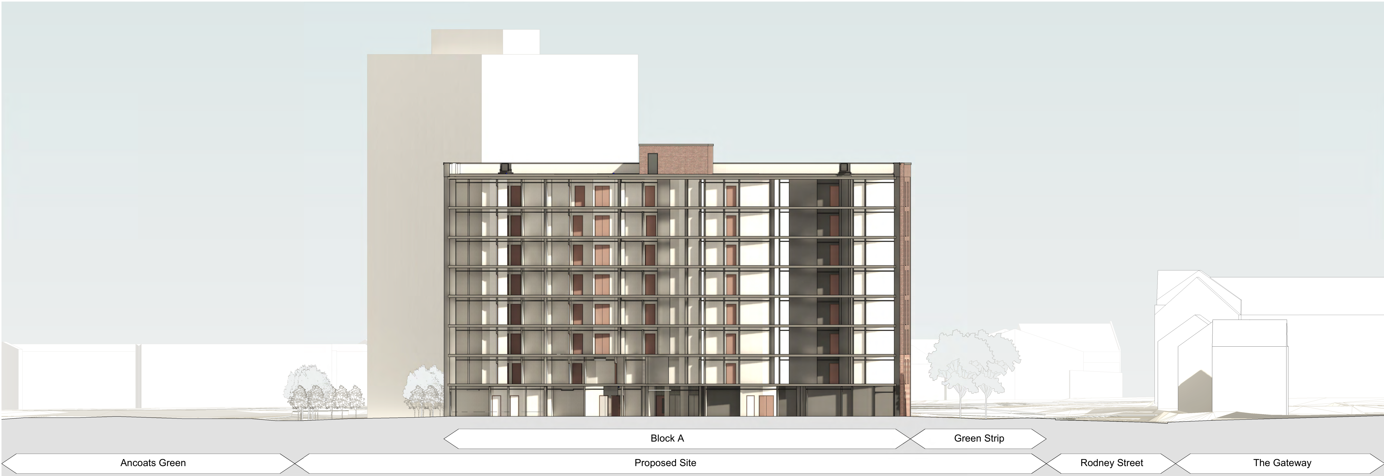
Proposed Site Section AA 1 : 200
