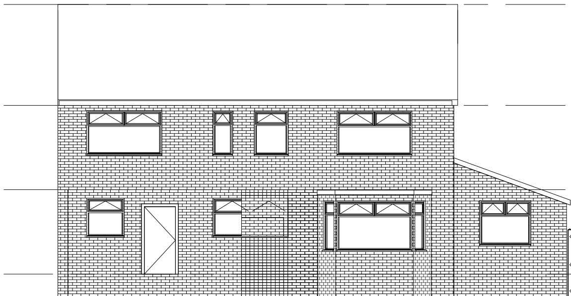
2 Proposed Rear Elevation 1 : 100
