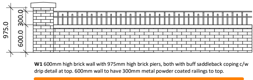
Boundary details 1 : 50
