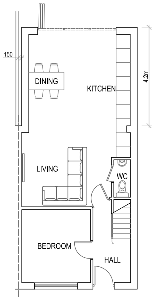
PROPOSED GF PLAN 1:100
