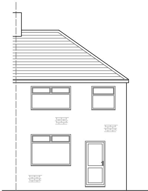
PROPOSED FRONT ELEVATION 1:100
