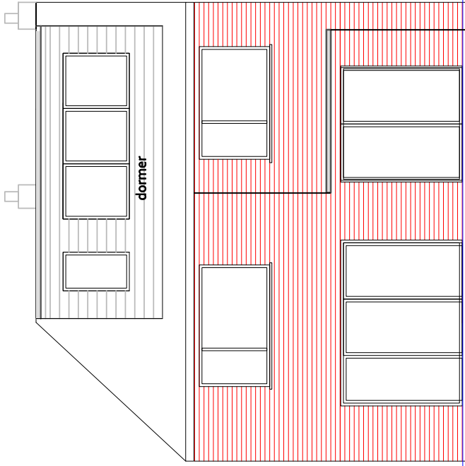
Proposed South Elevation
