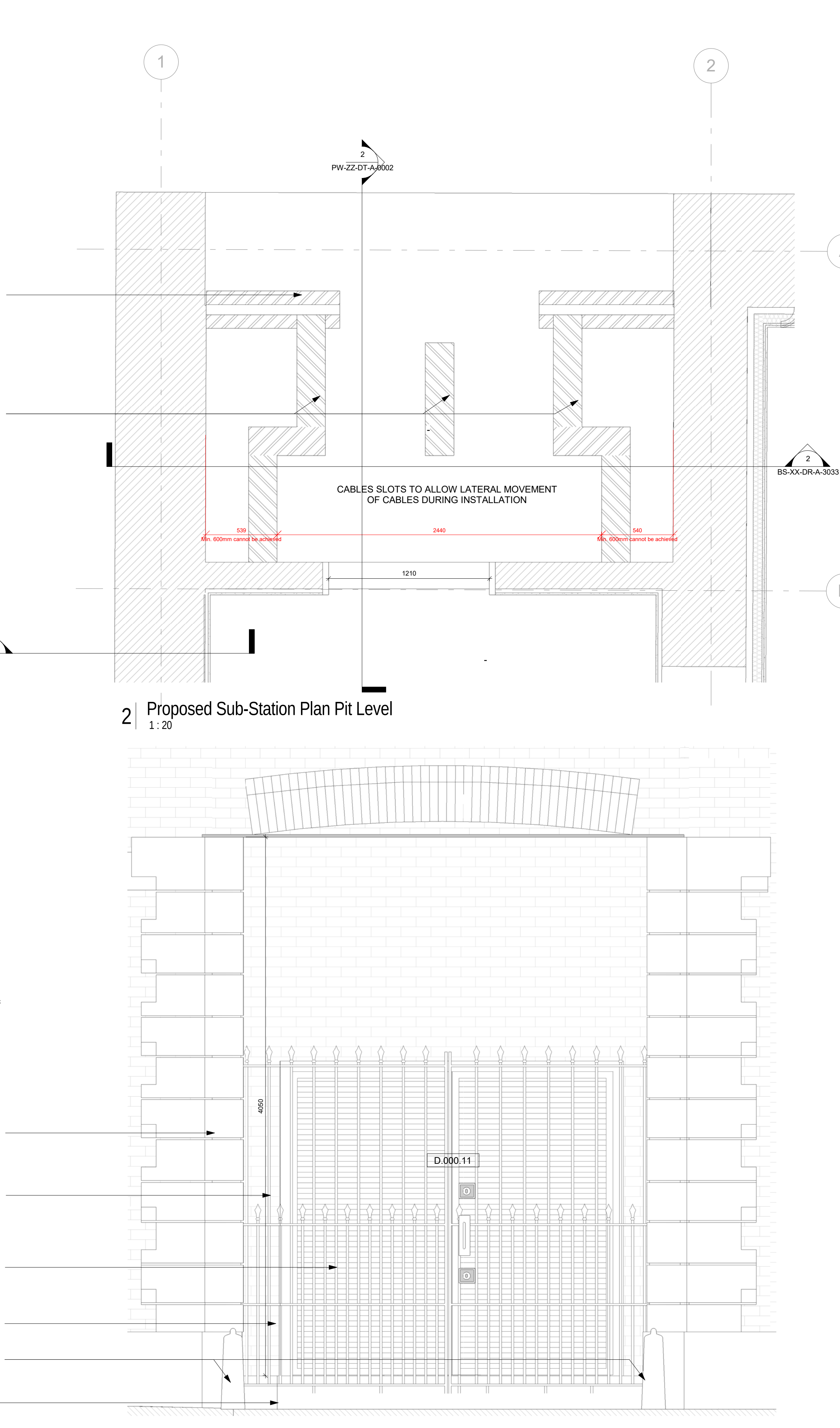
3 | Proposed Sub-Station Door Elevation
