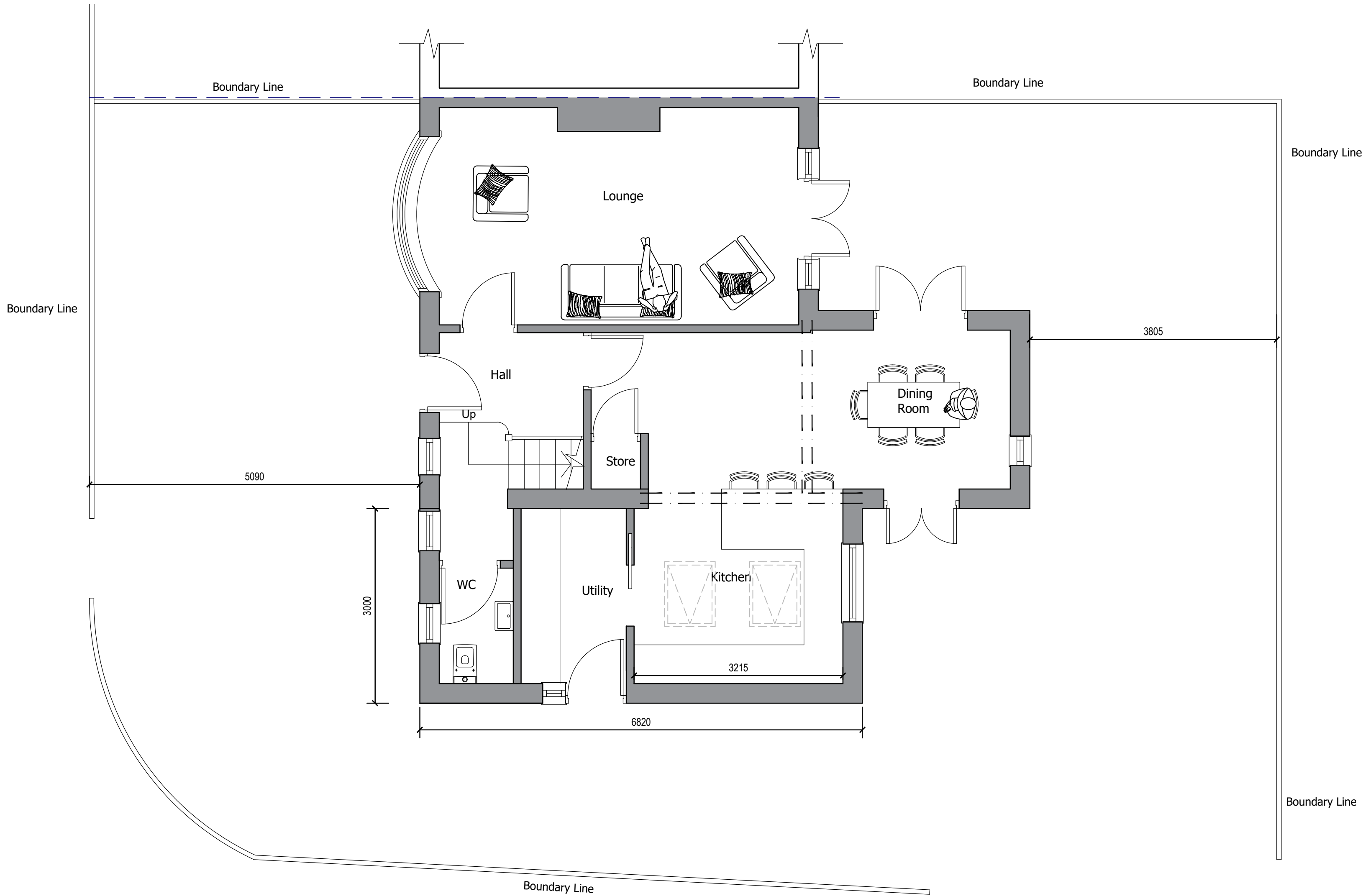
Ground Floor
