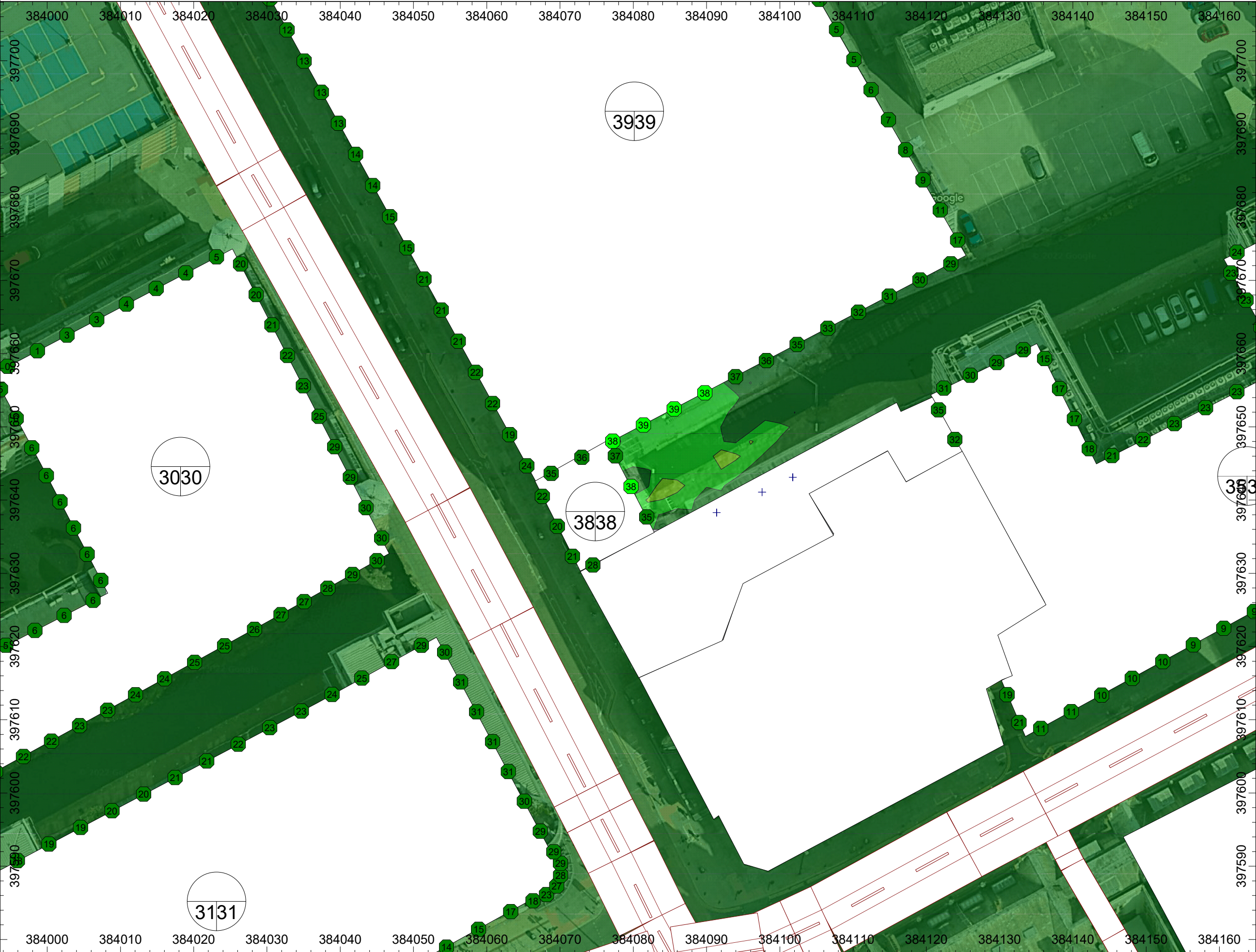
Figure 2 - Fixed Plant Sound Grid Noise Map - Calculation at 15m above ground level
