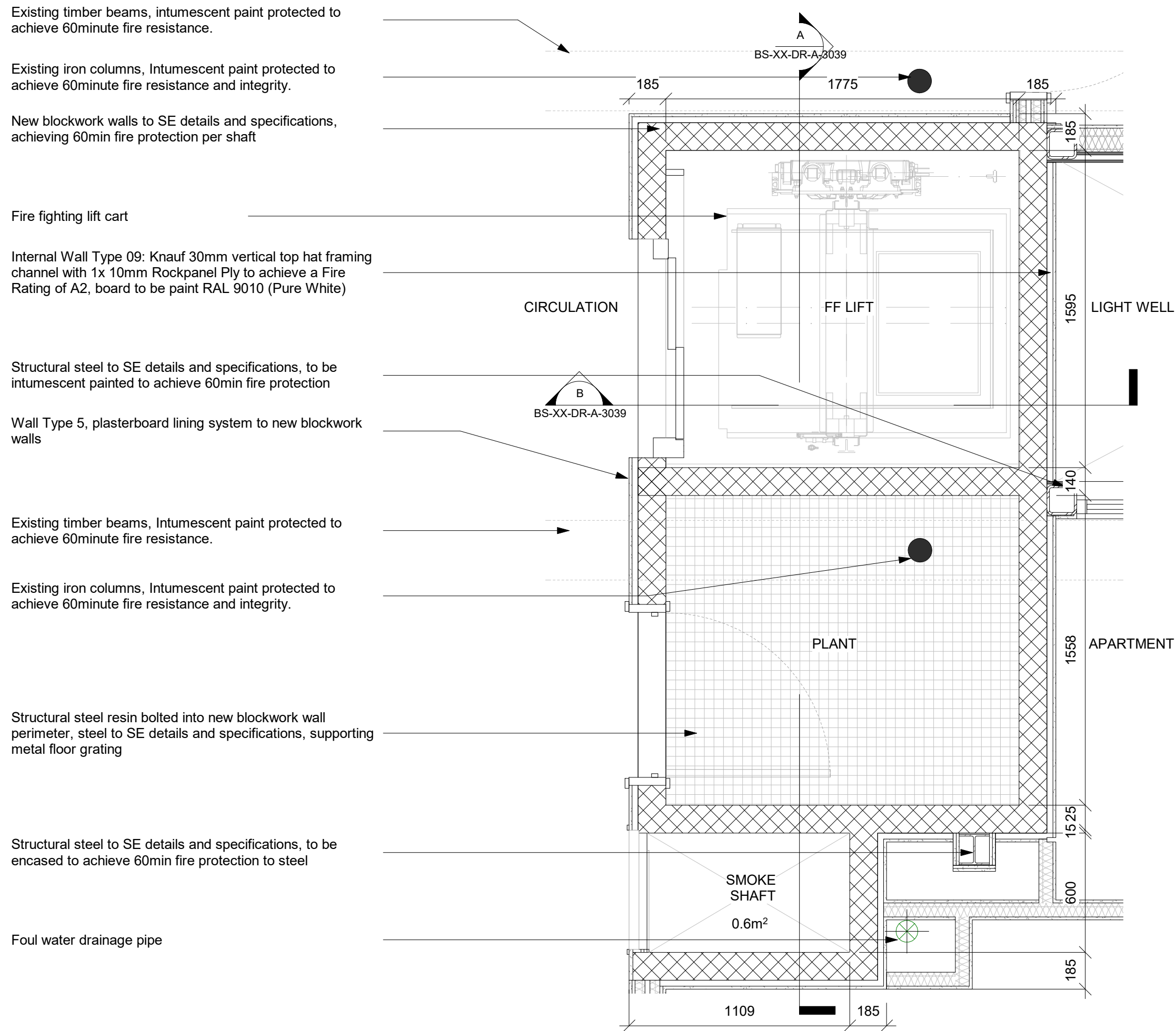
PL | TYPICAL LIFT CORE PLAN 1 : 20
